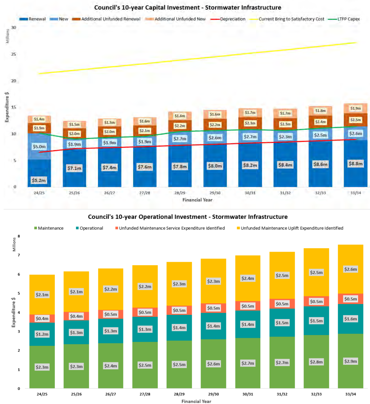
Figure 10 Stormwater Asset Expenditure
