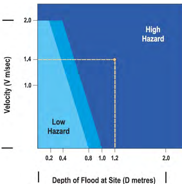
Figure 8-5 Provisional Hazard Classification (NSW Government)
