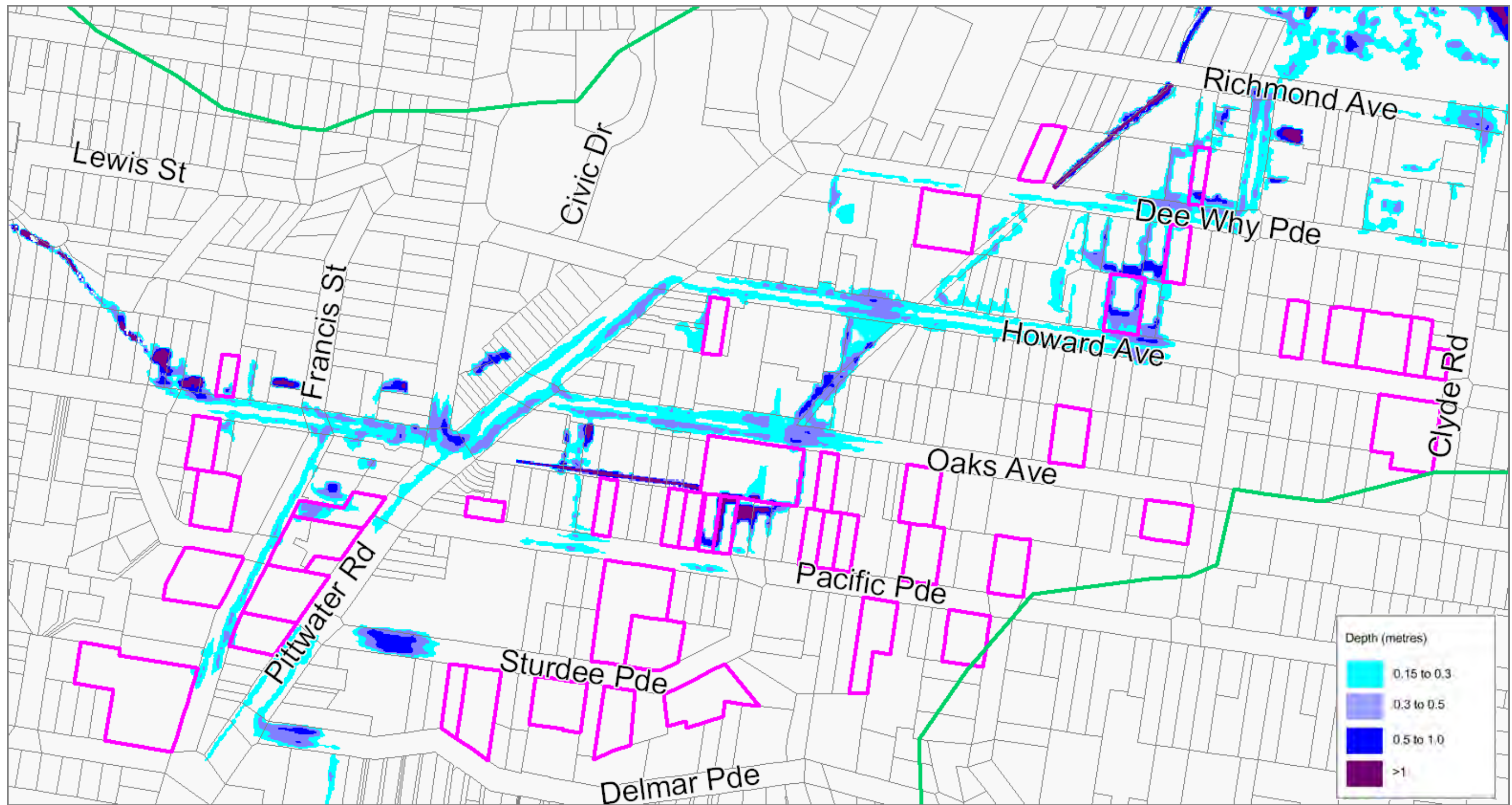
Figure 6-19 Basement Car Park – Peak Depths 1% AEP
