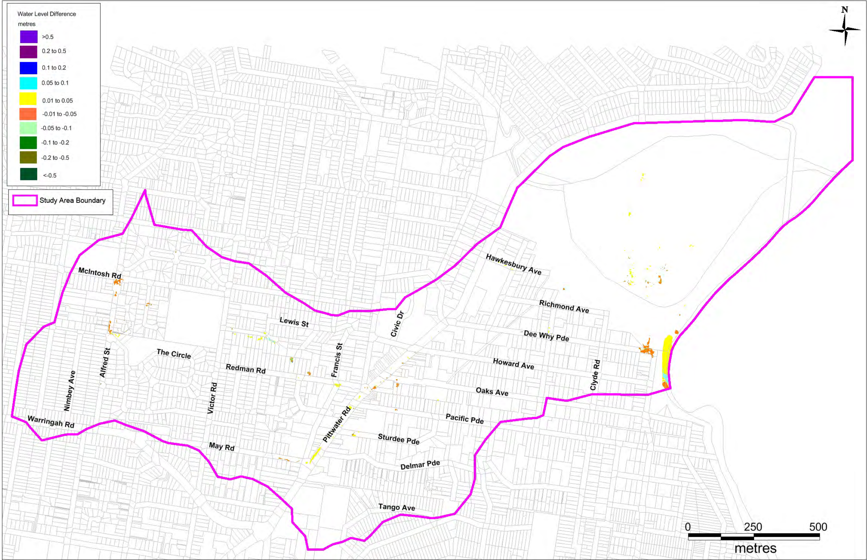
Figure 7-1 Sensitivity – Surface Roughness +20%
