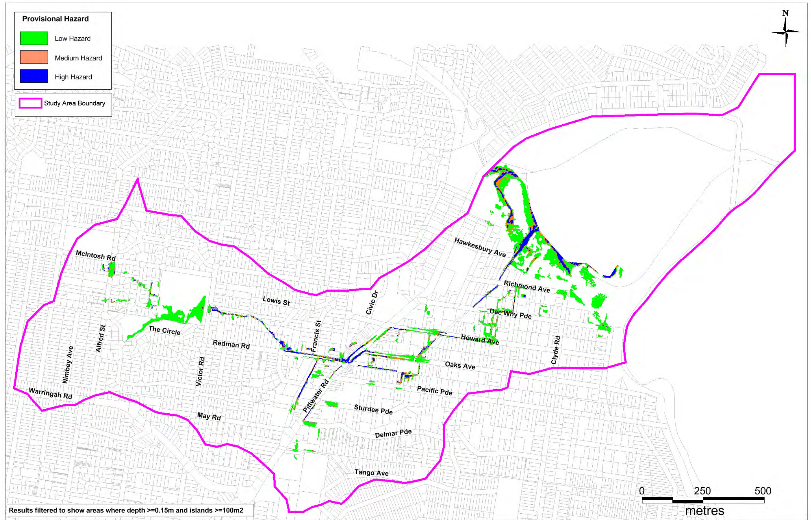
Figure 8-8 Provisional Hazard Classification 5% AEP Event
