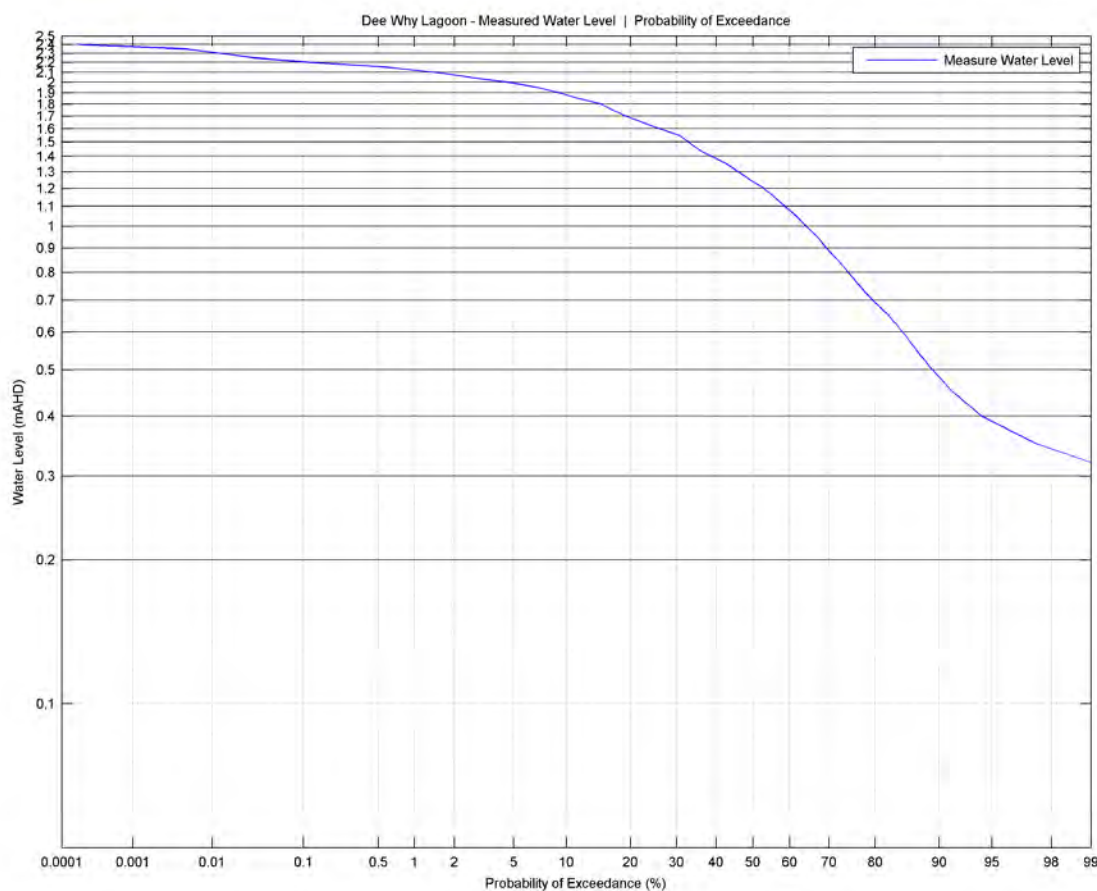
Figure 10-2 Dee Why Lagoon Probability of Exceedance (1996-2012)
