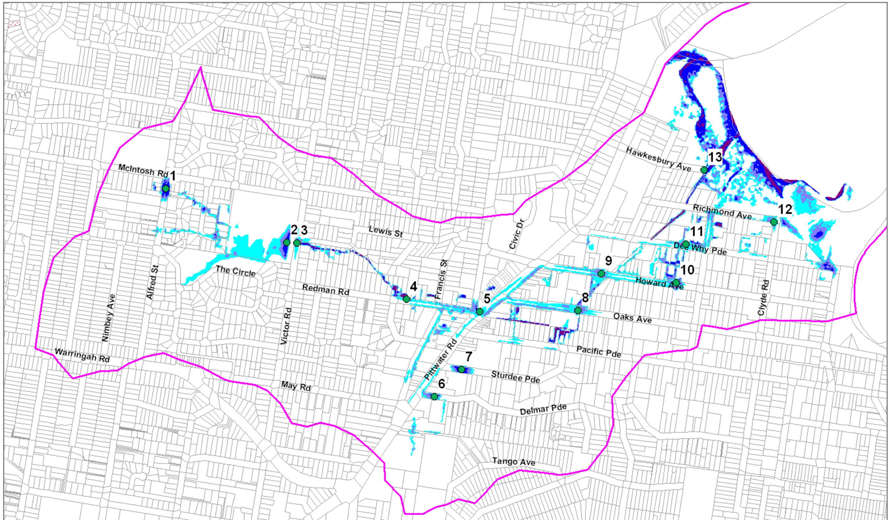
Figure 6-17 Peak Flood Level Reference Locations
