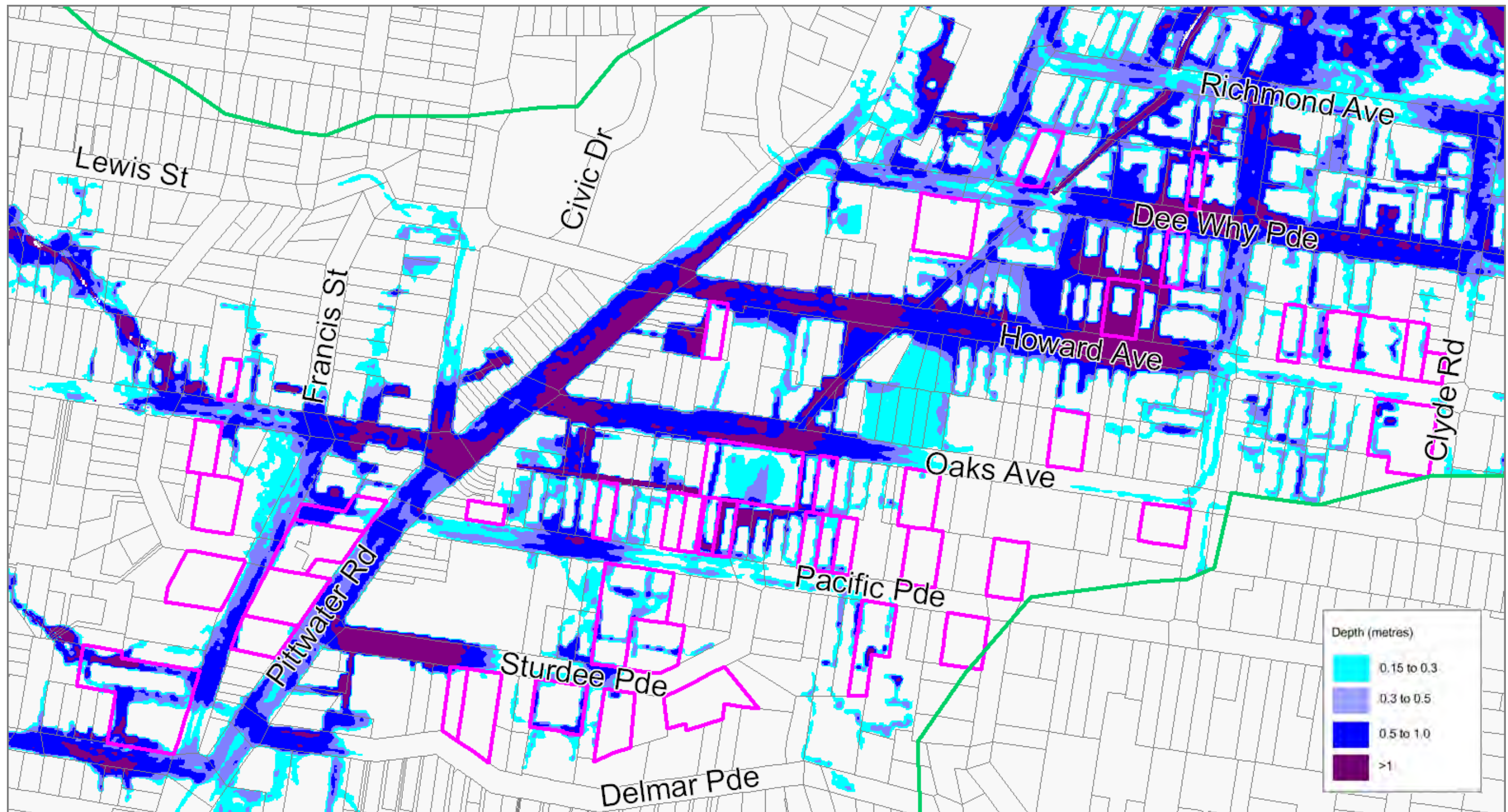
Figure 6-20 Basement Car Park – Peak Depths PMF
