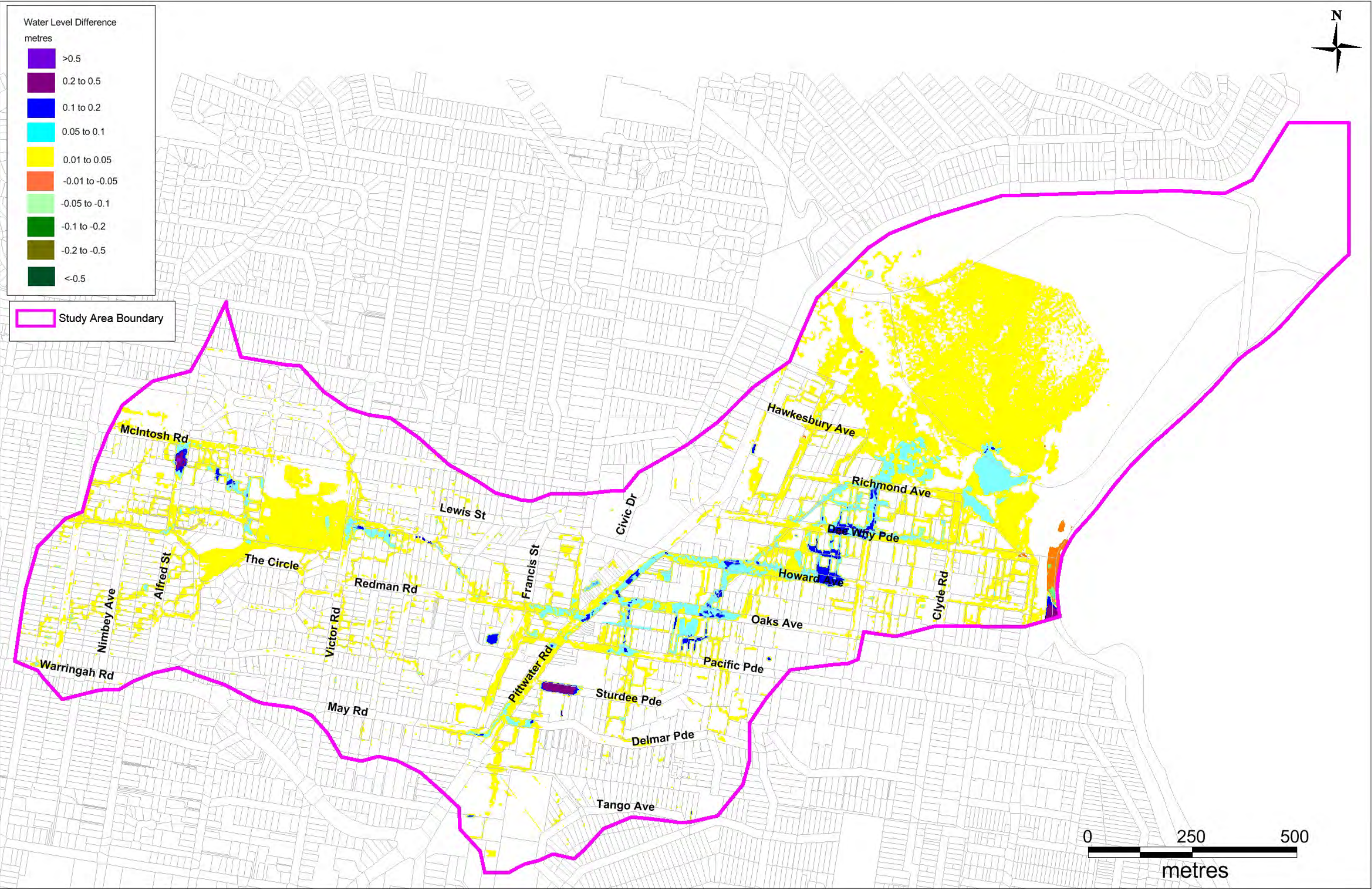
Figure 11-4 Rainfall Intensity Increase 20%
