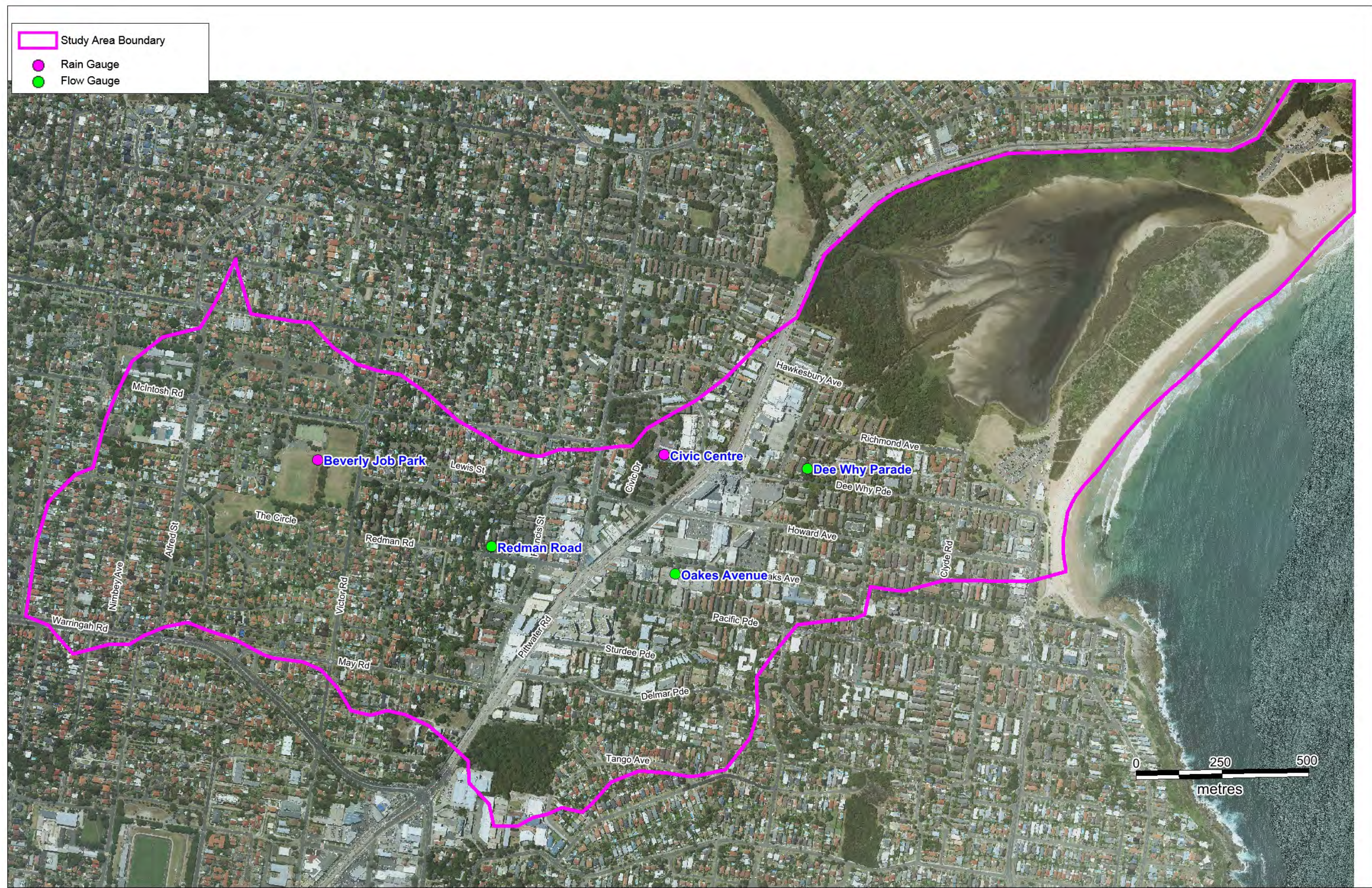
Figure 2-7 Approximate Locations of Rain and Flow Gauges
