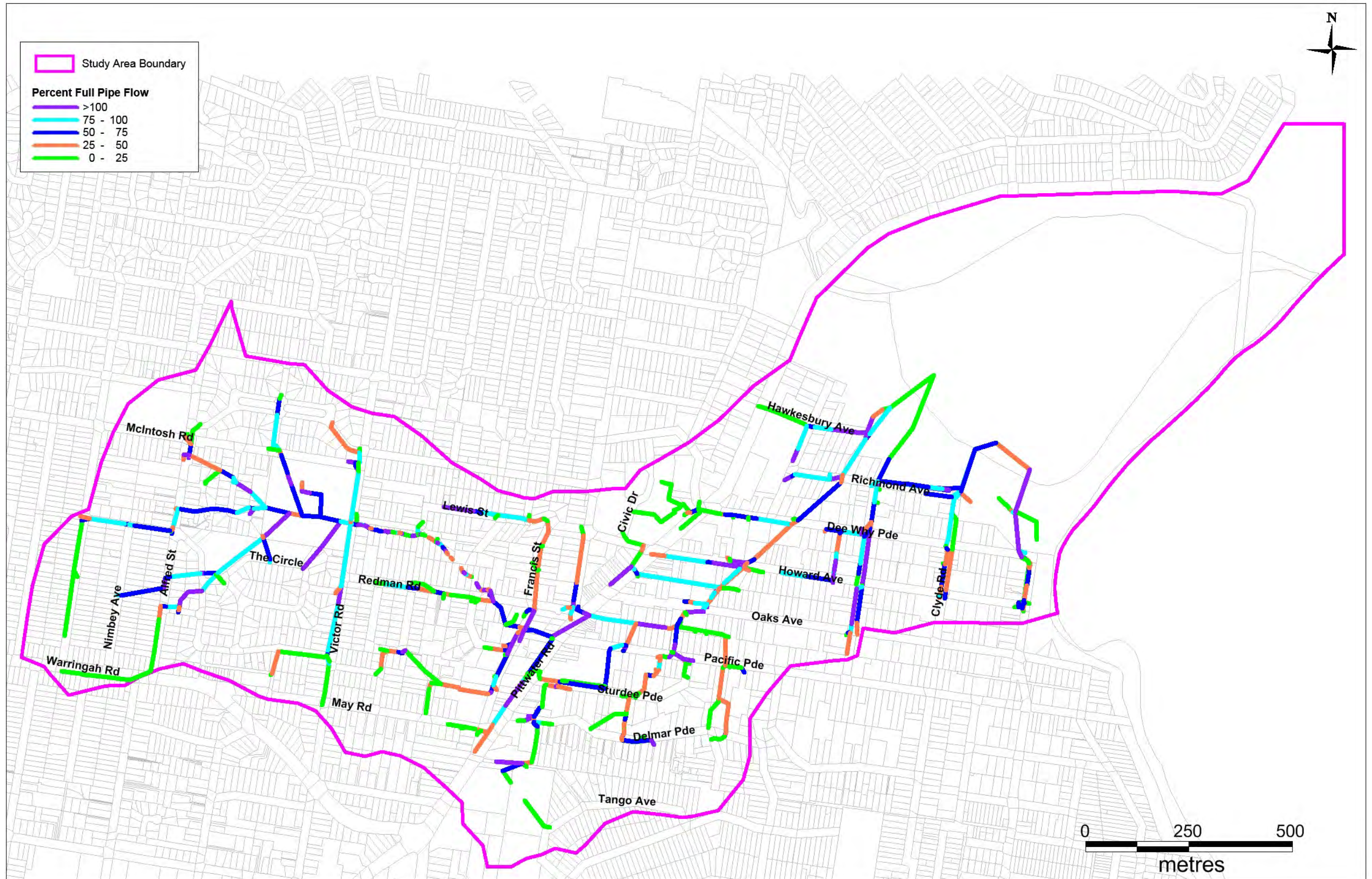
Figure 9-2 Stormwater Infrastructure Capacity – % Capacity in 5 Year ARI
