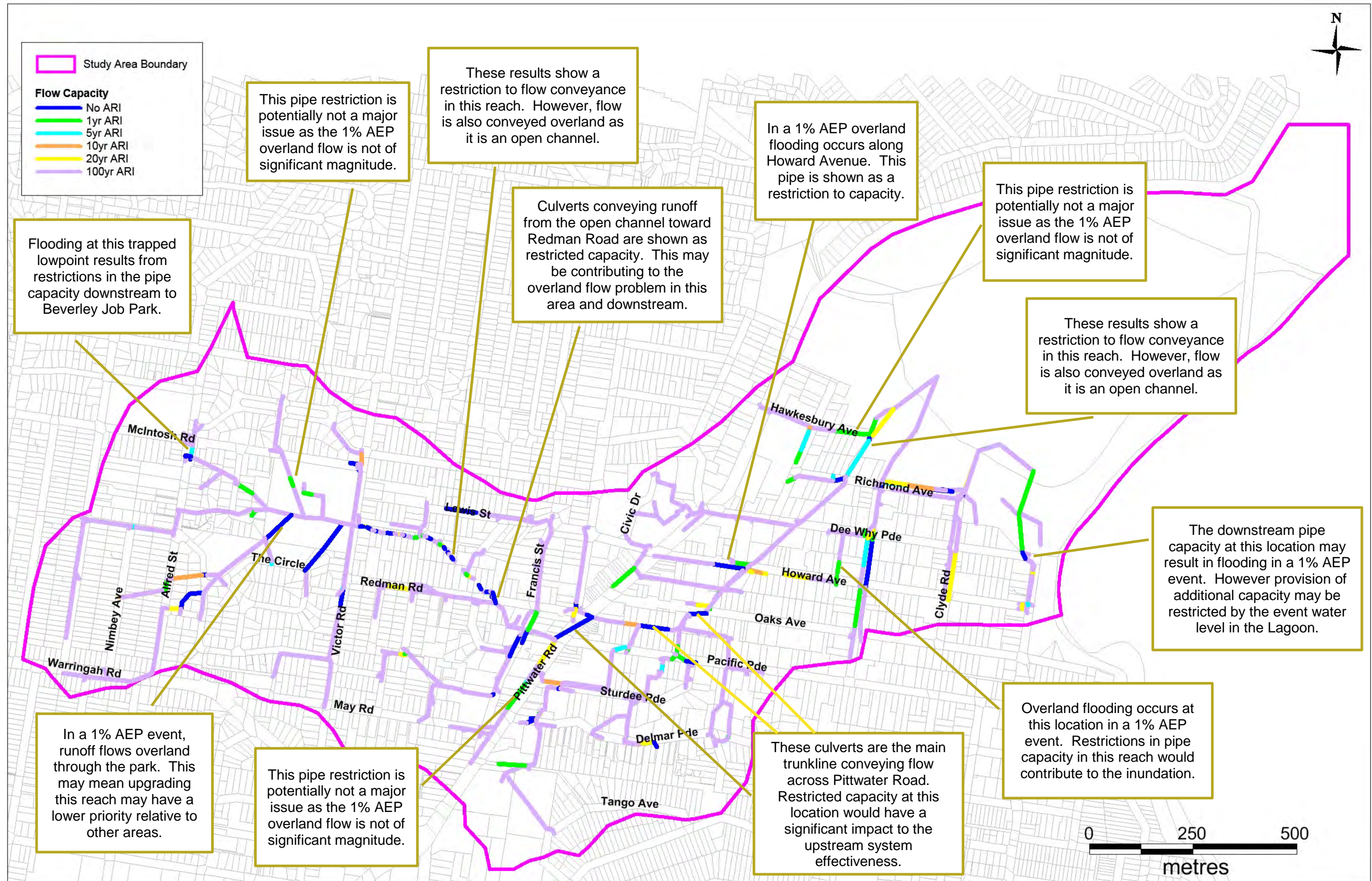
Figure 9-3 Review of Stormwater Infrastructure Capacity
