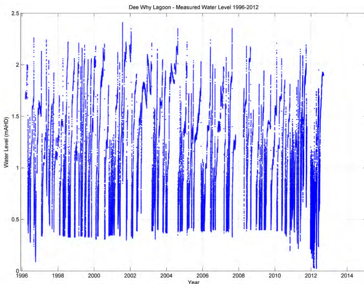
Figure 10-1 Dee Why Lagoon Water Level Time Series (1996-2012)
