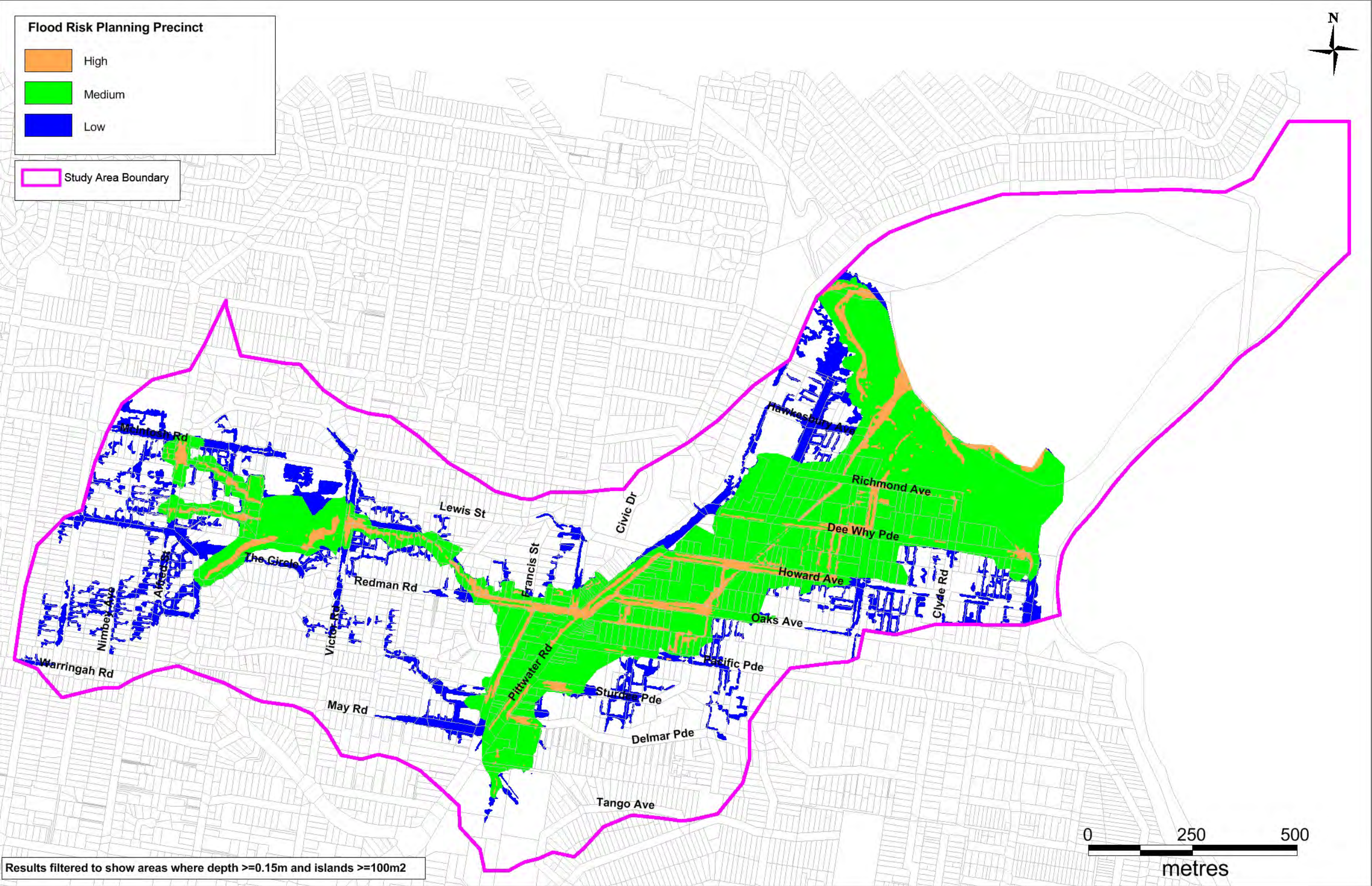
Figure 12-2 Flood Risk Planning Precincts
