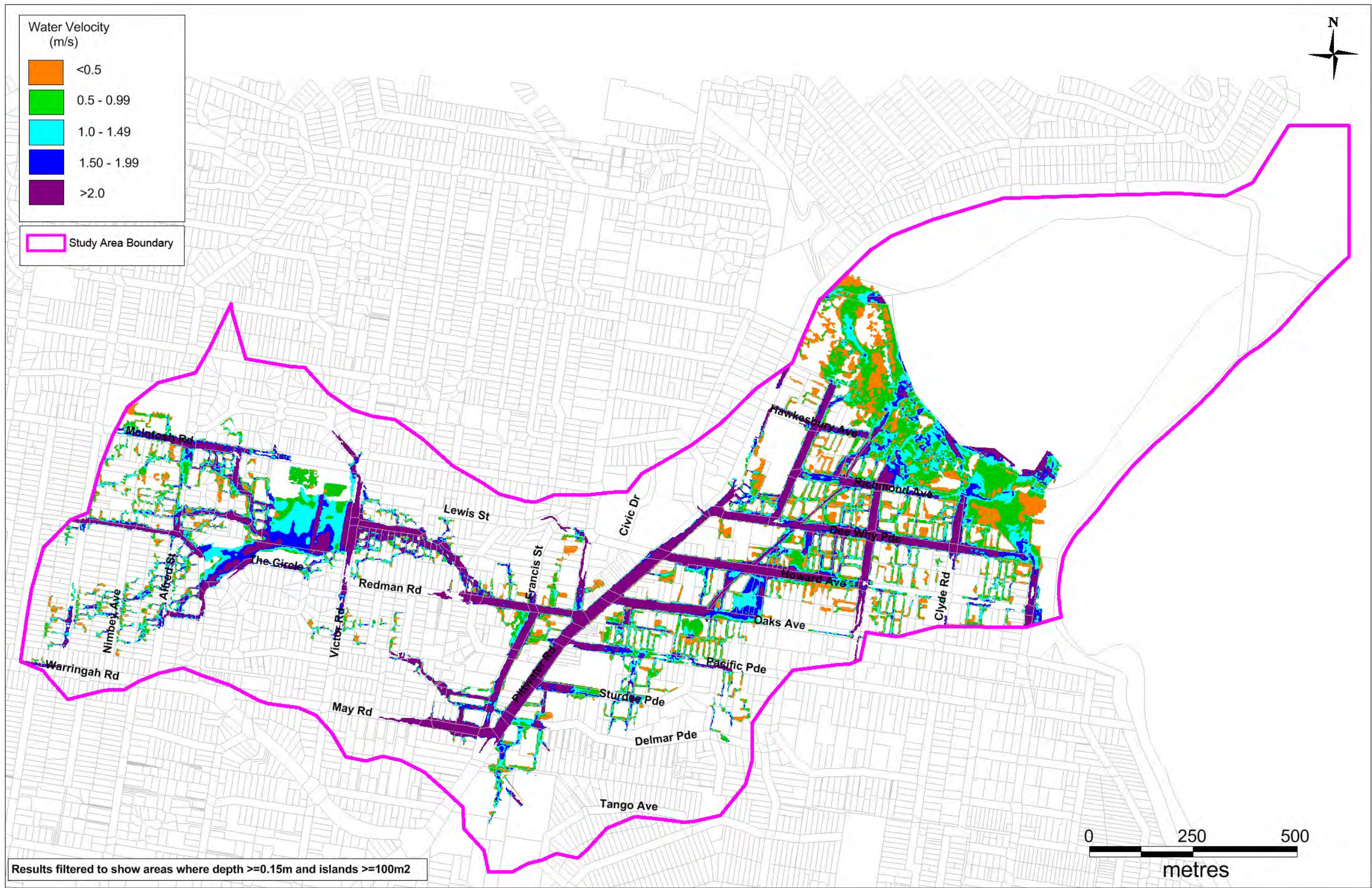
Figure 6-2 Design Event PMF Peak Velocity
