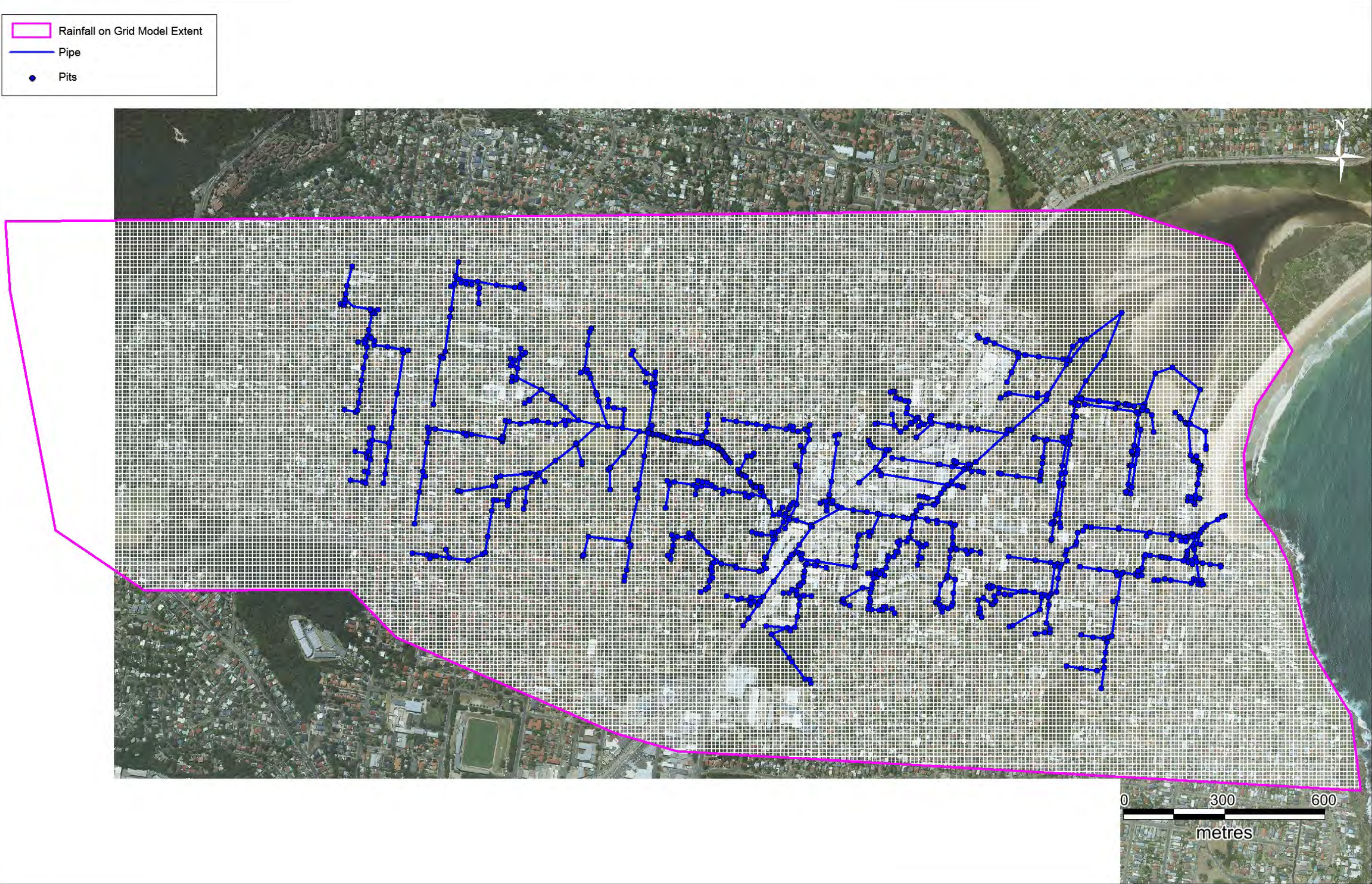
Figure 2-2 Rainfall-on-Grid XP-SWMM Model Layout (Cardno)
