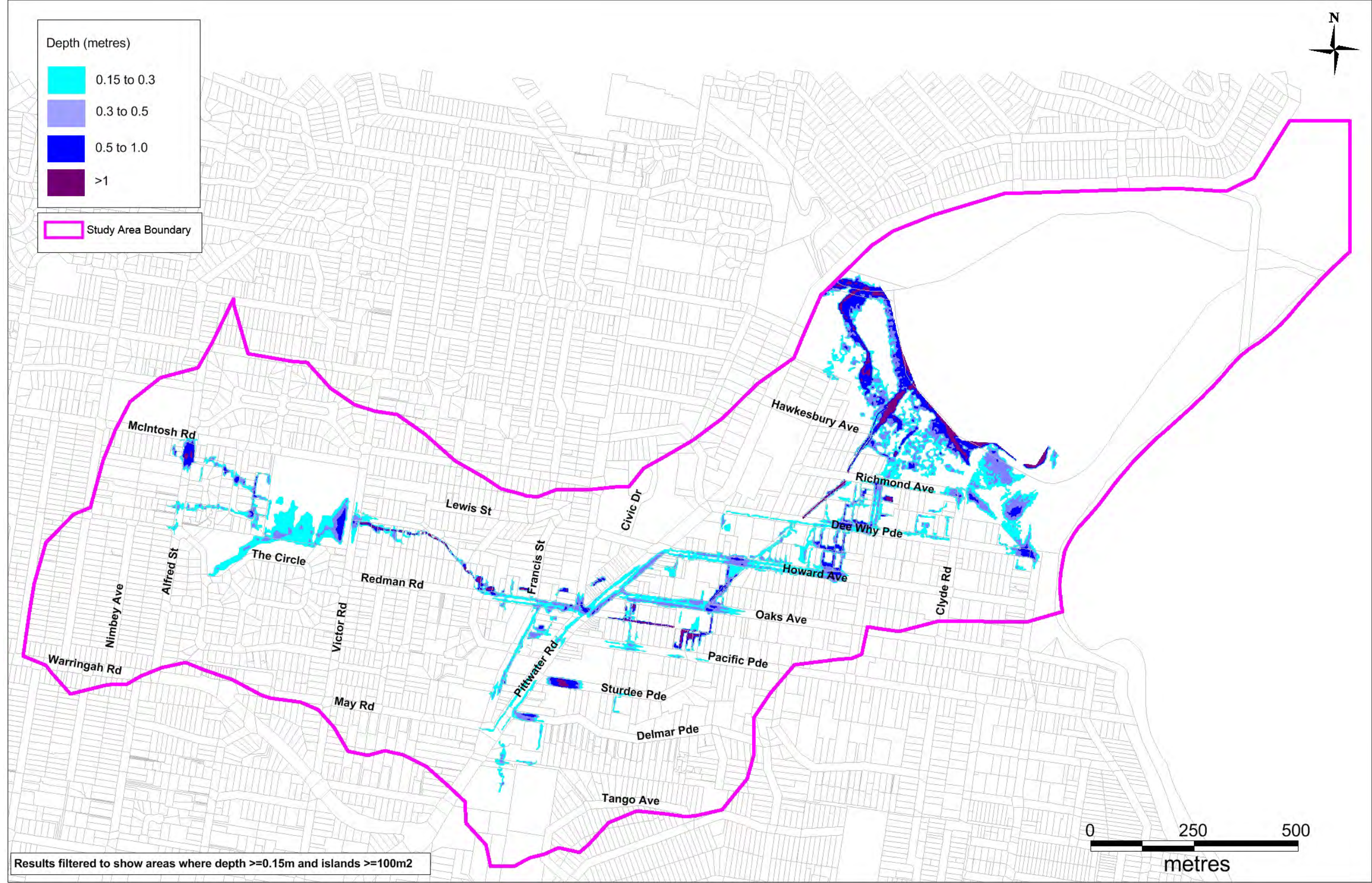
Figure 6-5 Design Event 0.5% AEP Peak Depth
