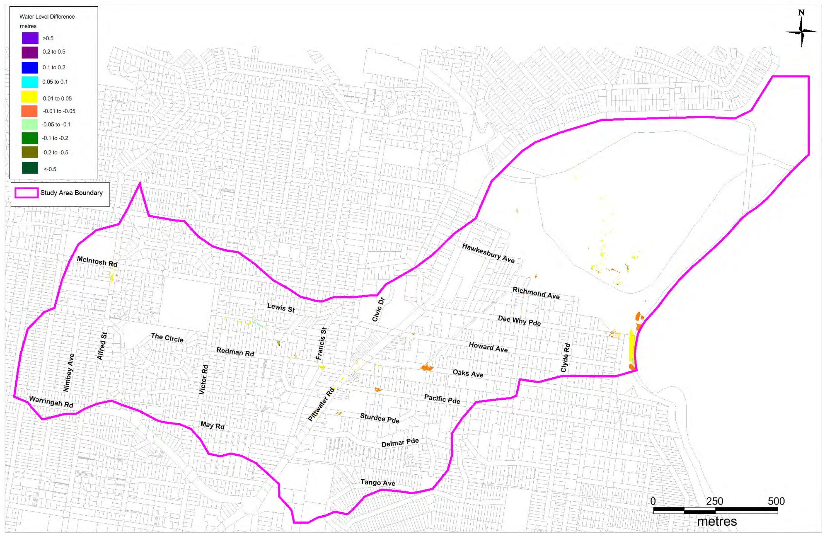
Figure 7-9 Sensitivity – Unlimited Inlet Capacity (0% Blockage)
