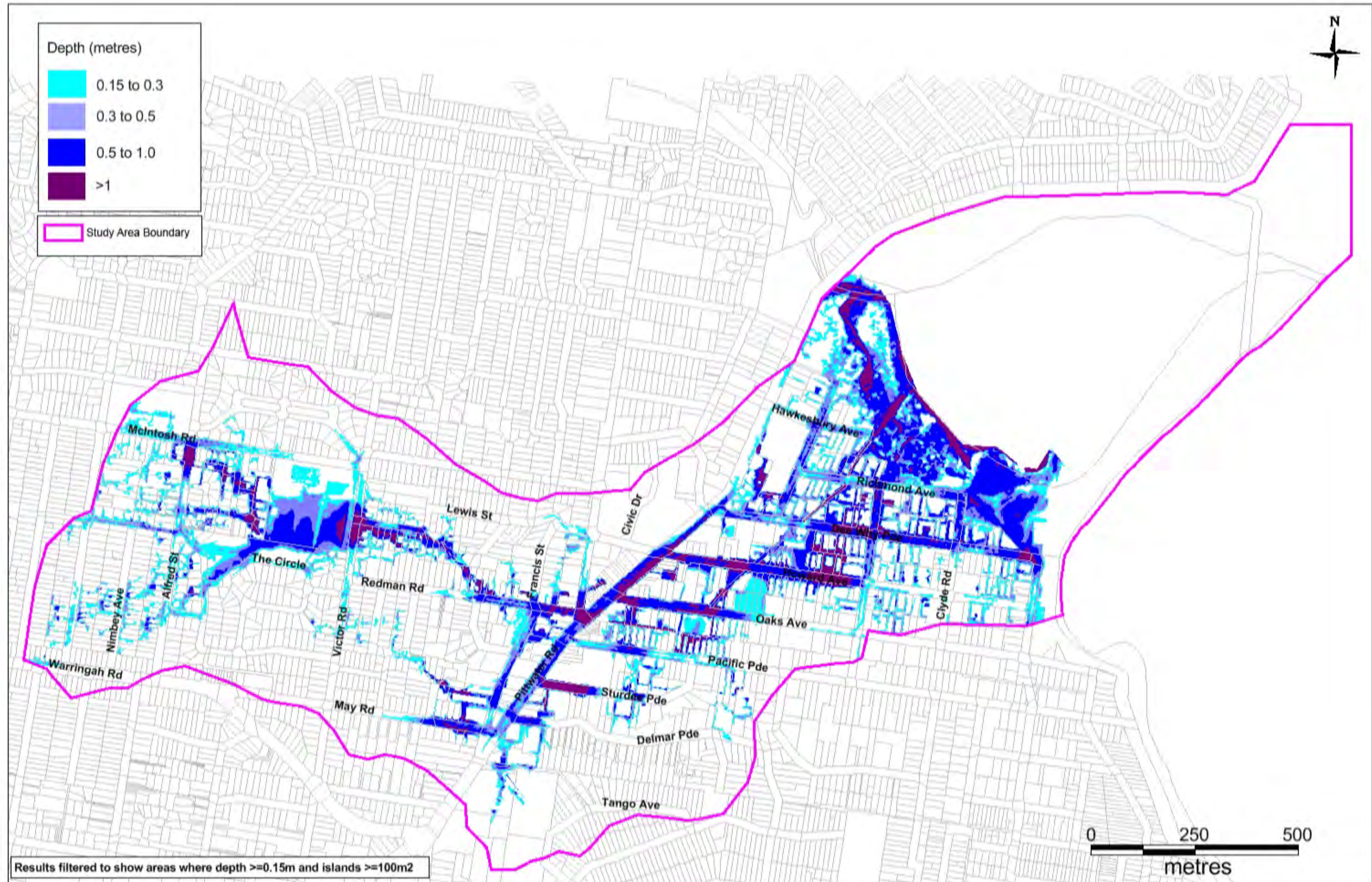
Figure 6-1 Design Event PMF Peak Depth
