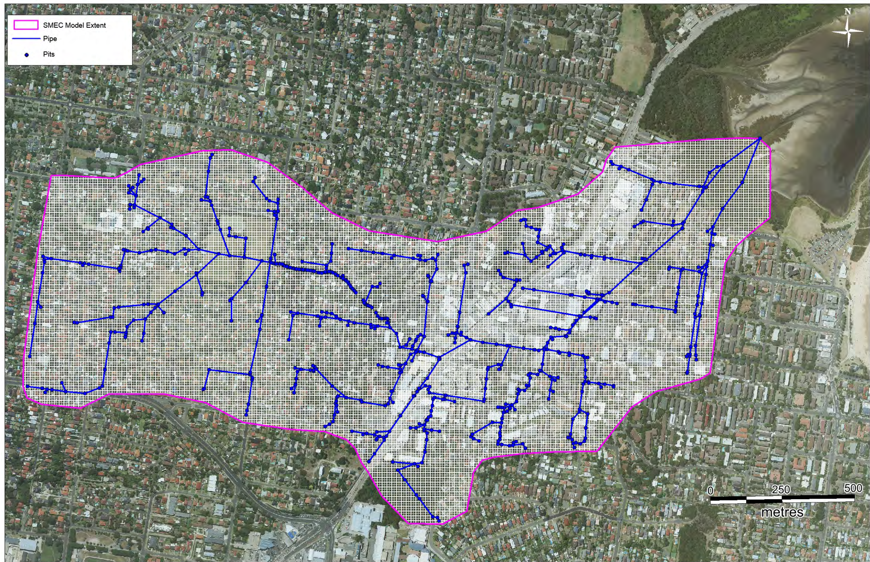
Figure 2-1 General Layout of the SMEC XP-SWMM Model
