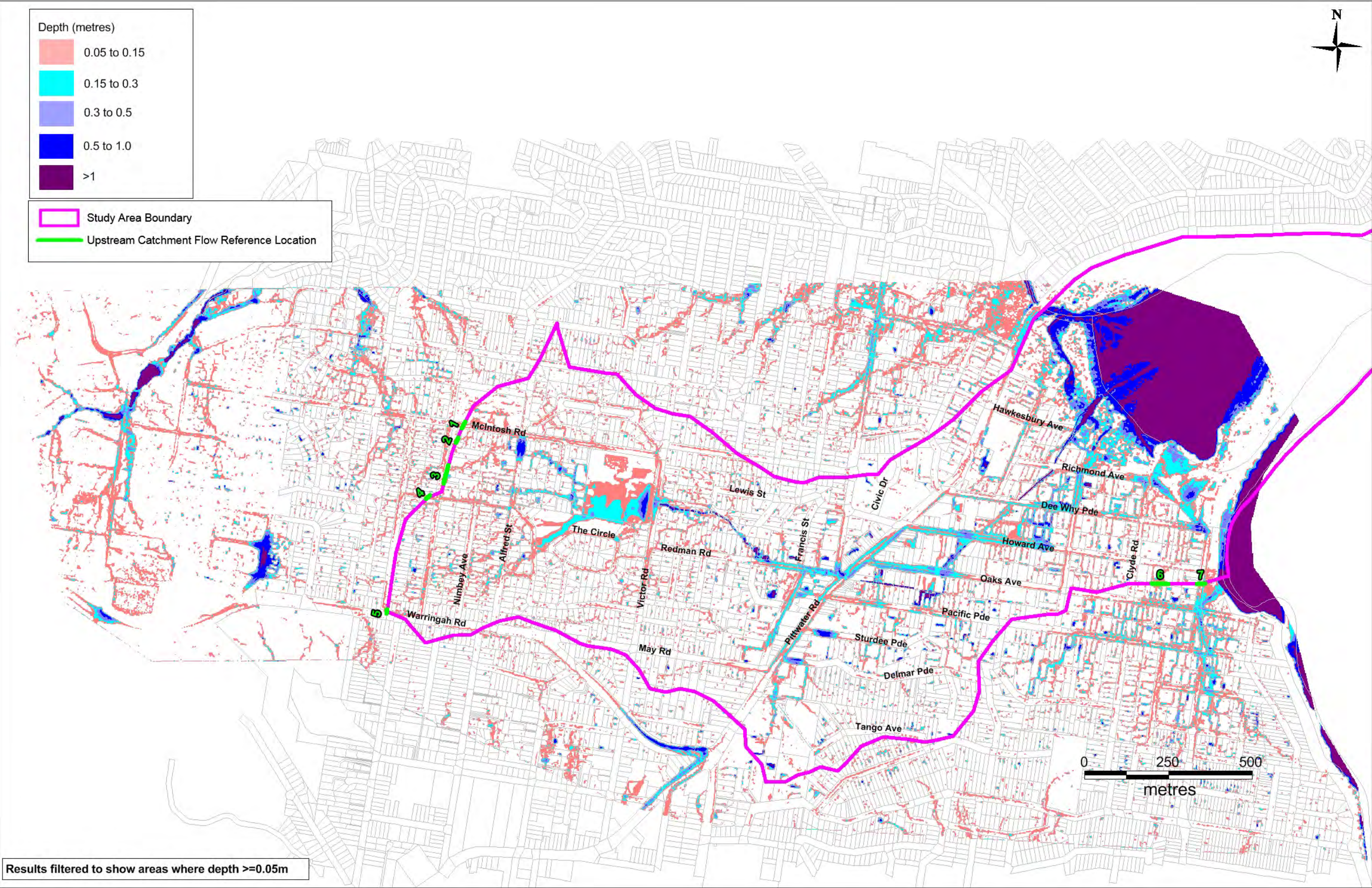
Figure 5-3 1% AEP External Catchment Extent
