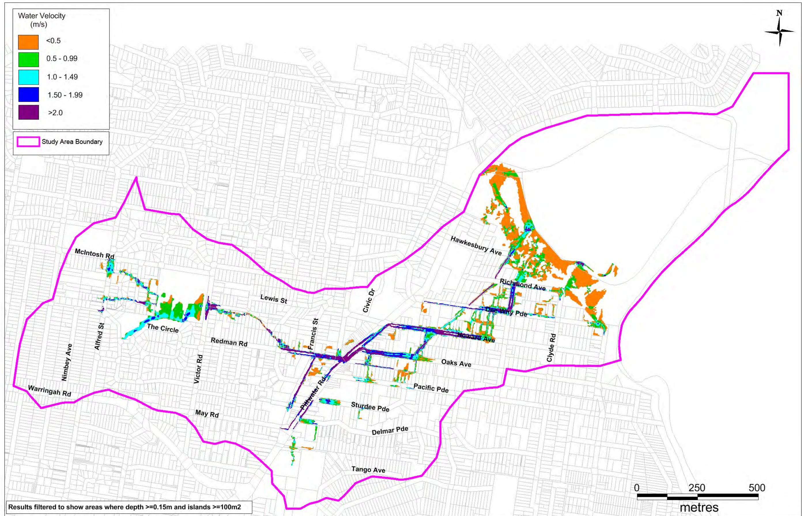
Figure 6-6 Design Event 0.5% AEP Peak Velocity
