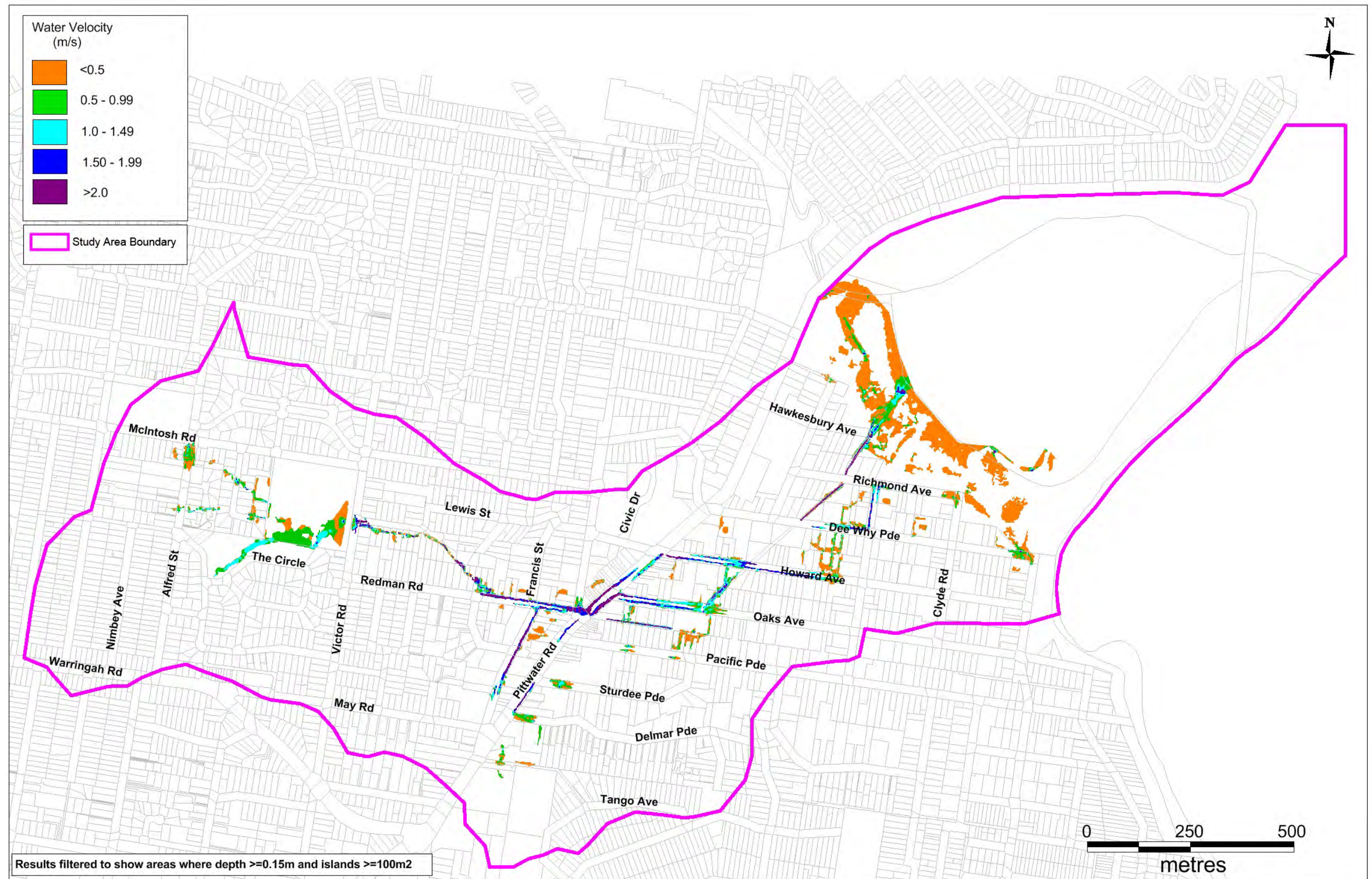
Figure 6-10 Design Event 5% AEP Peak Velocity
