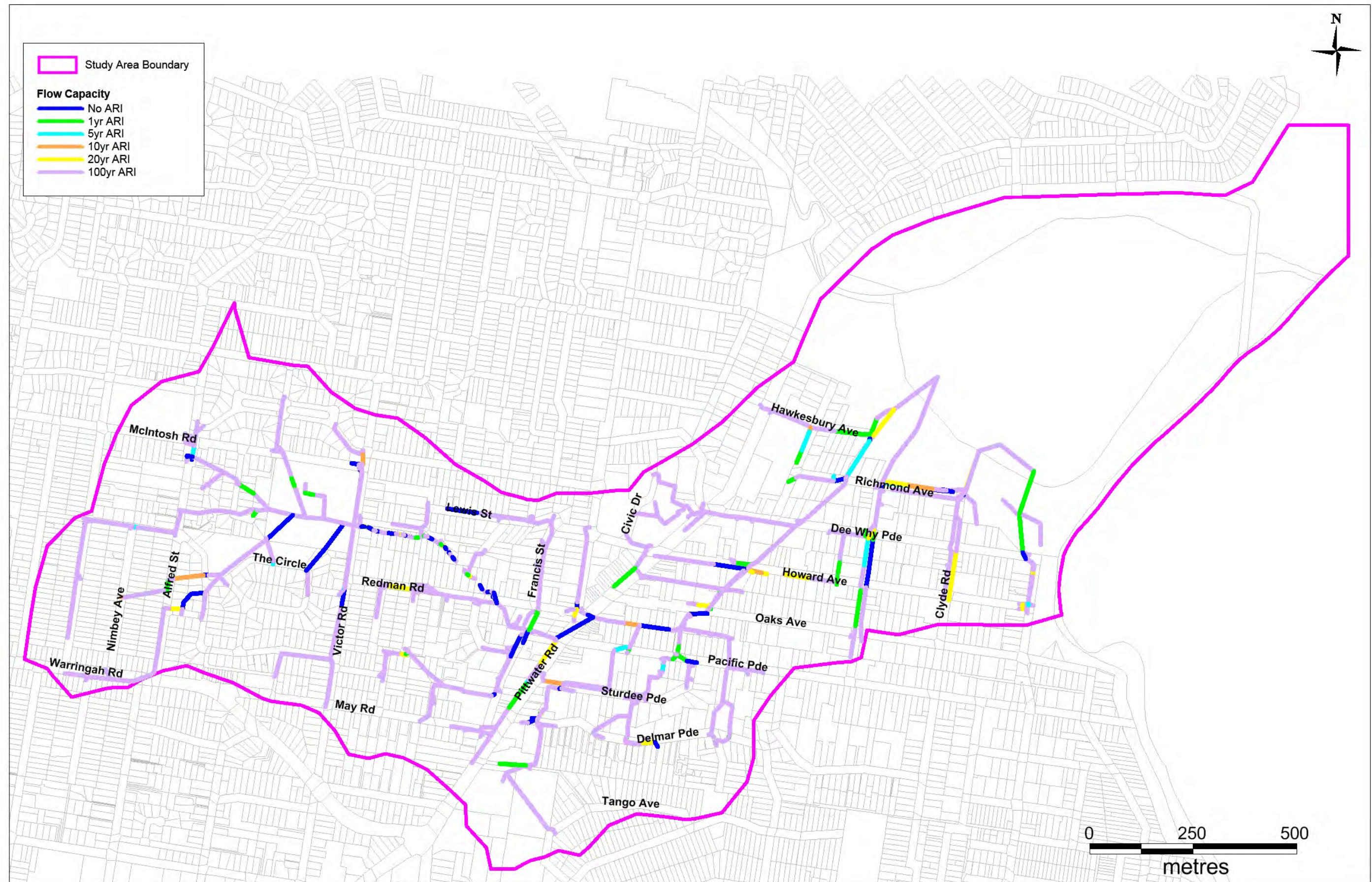
Figure 9-1 Stormwater Infrastructure Capacity – ARI Event to 100% Capacity
