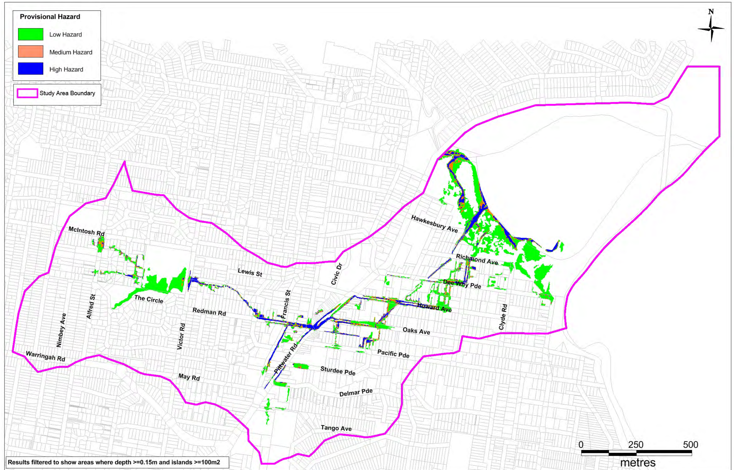
Figure 8-7 Provisional Hazard Classification 1% AEP Event
