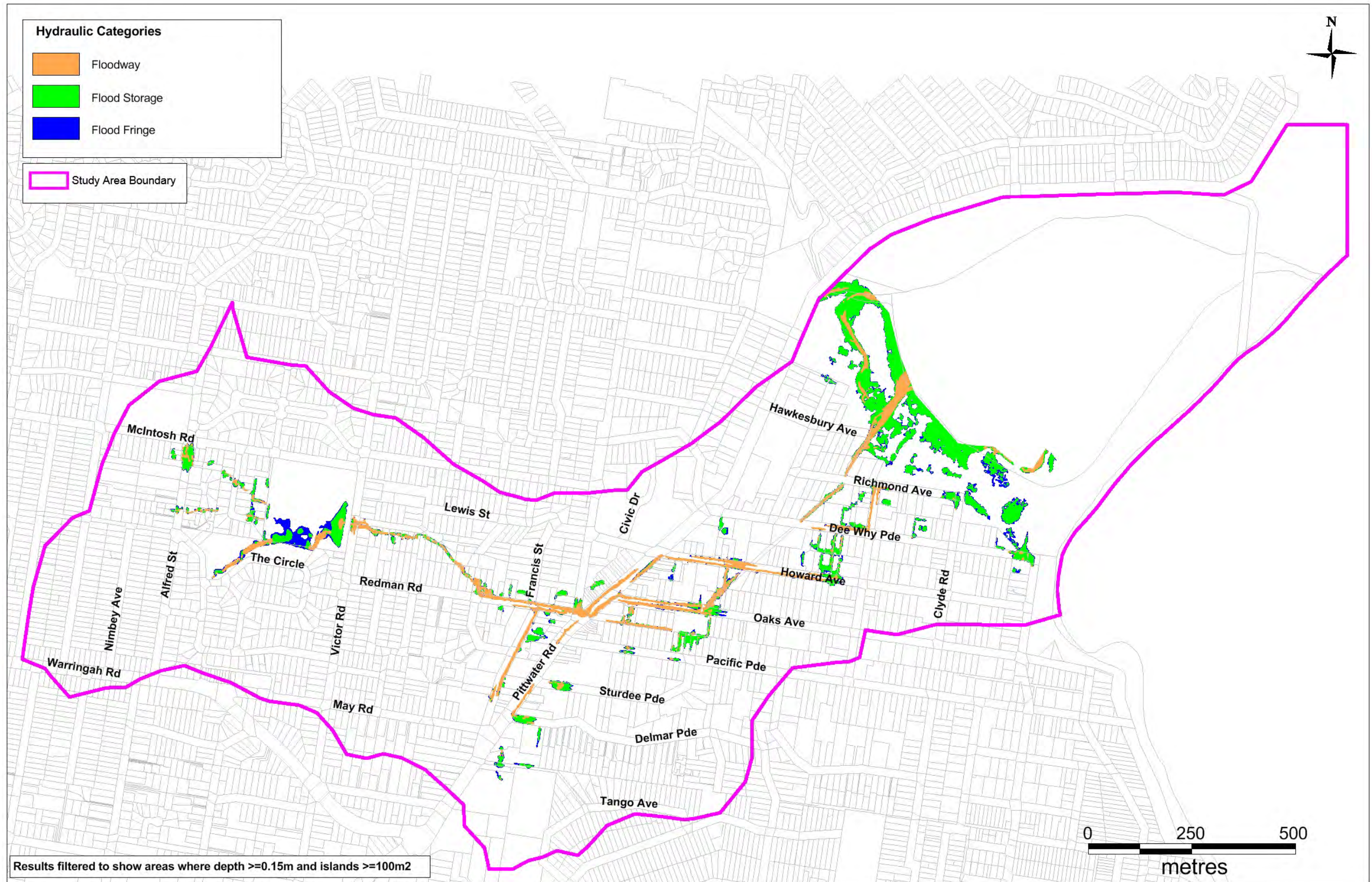
Figure 8-3 Hydraulic Categorisation 5% AEP Event
