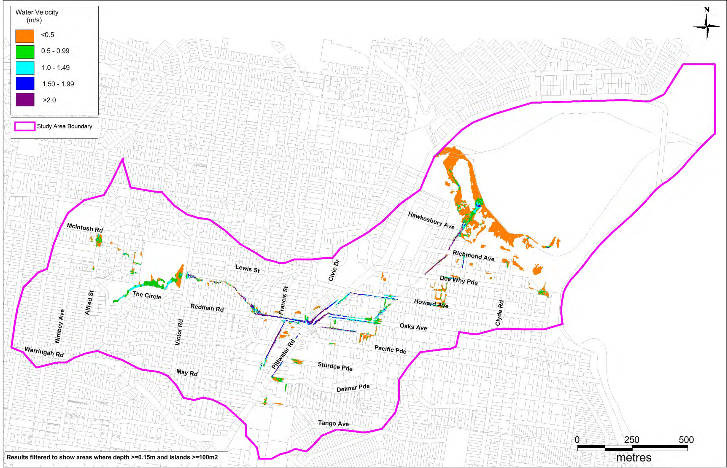
Figure 6-12 Design Event 10% AEP Peak Velocity
