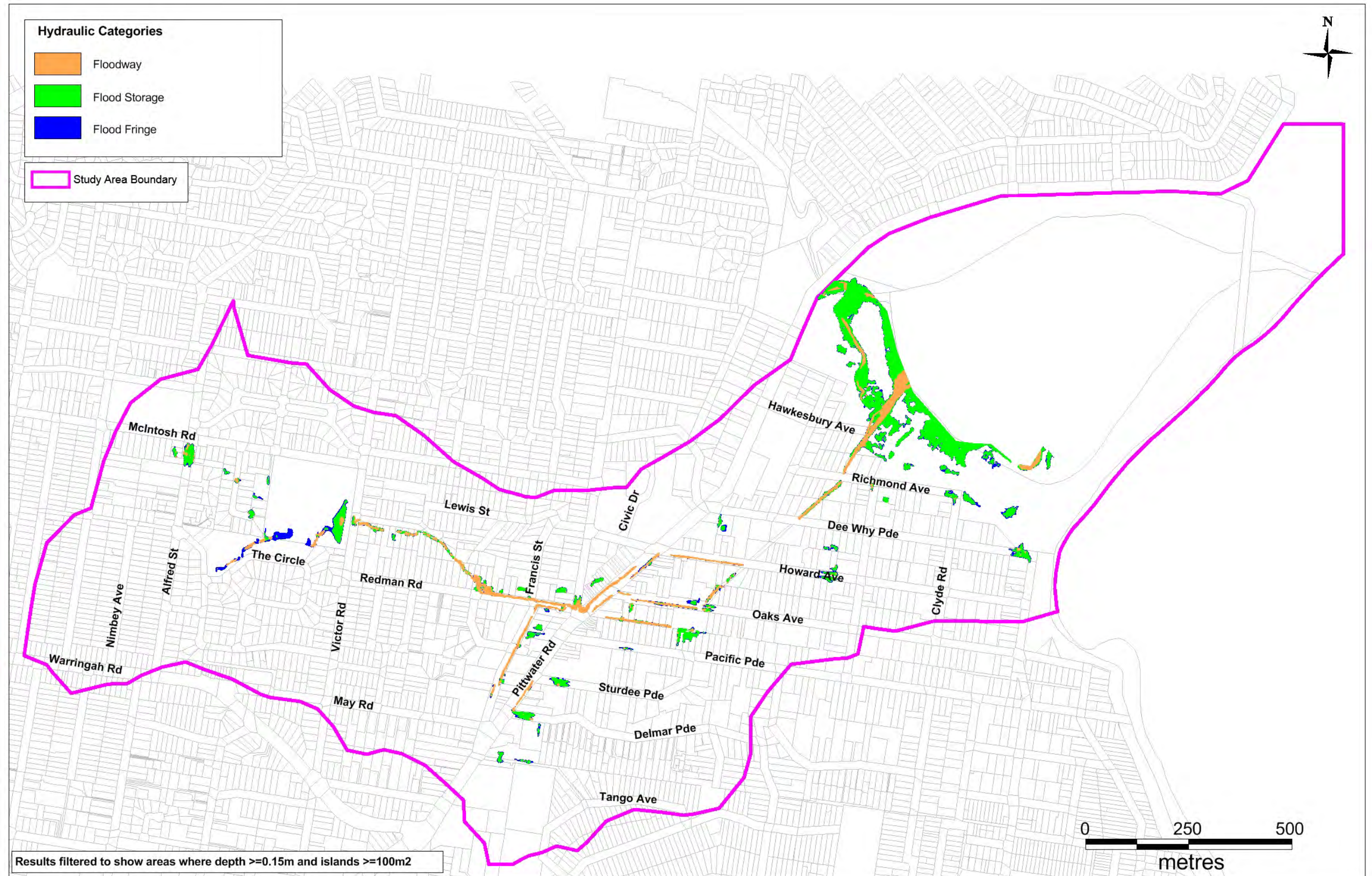
Figure 8-4 Hydraulic Categorisation 5 Year ARI Event
