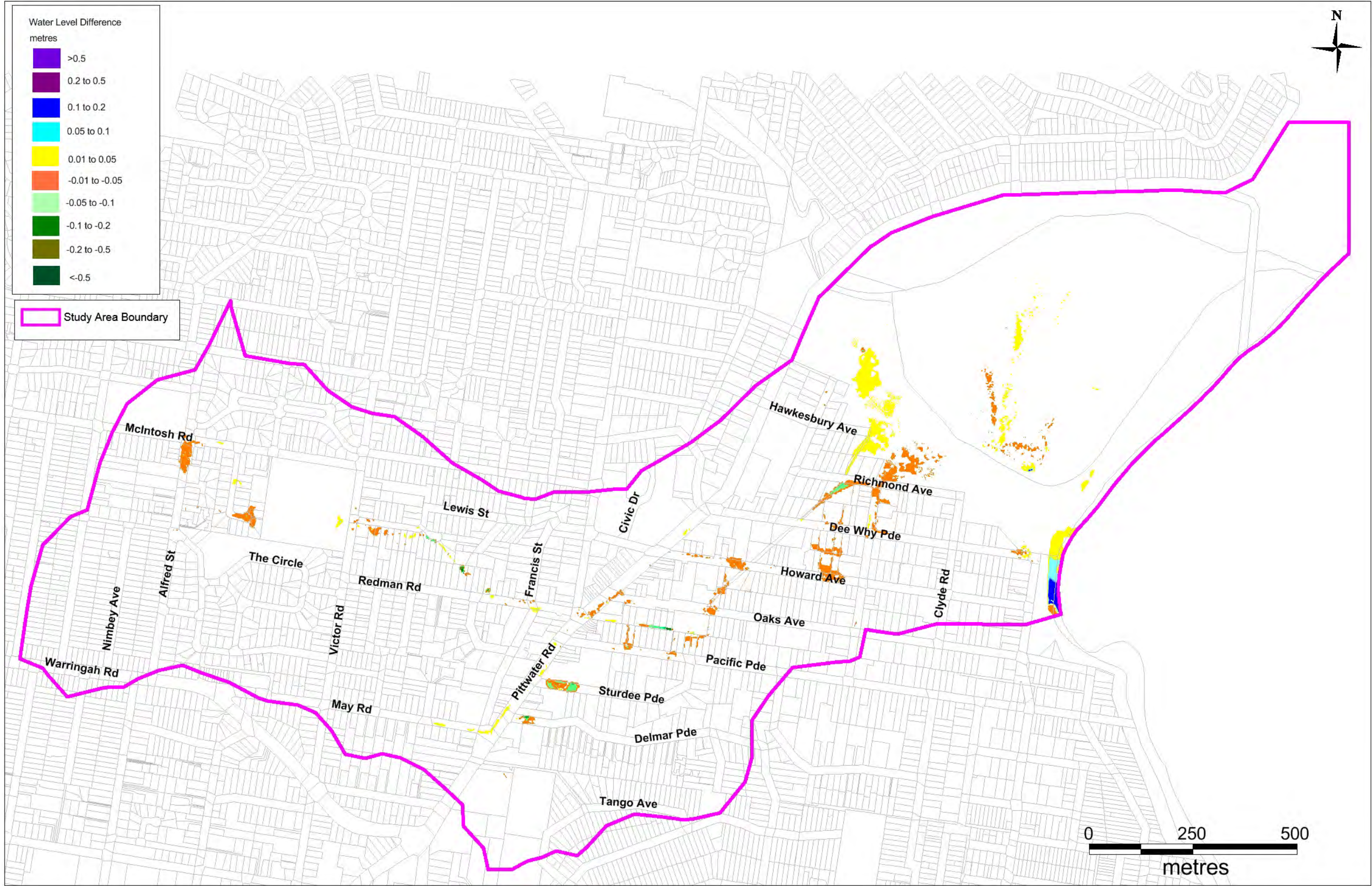
Figure 7-12 Sensitivity – Energy Losses at Structures -20%
