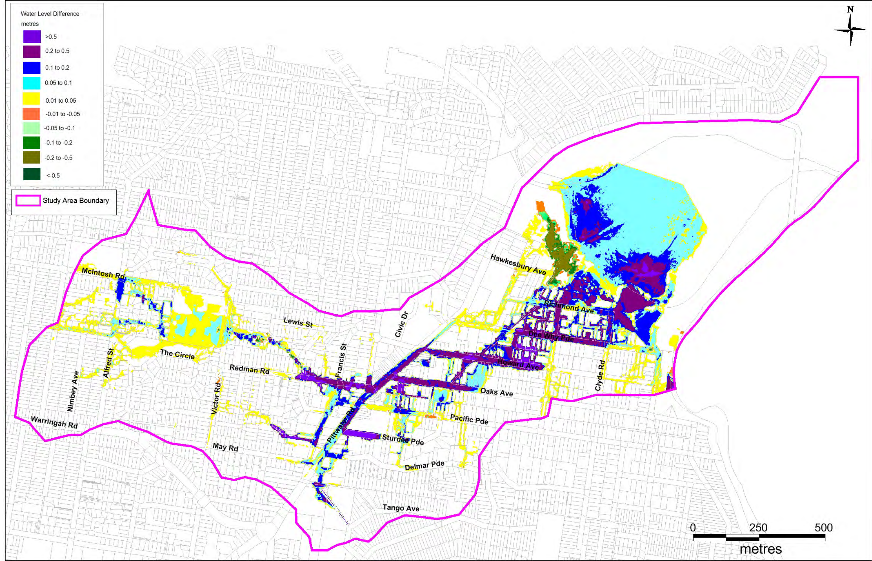
Figure 7-10 Sensitivity – Complete Inlet Blockage (0% Piped Conveyance)
