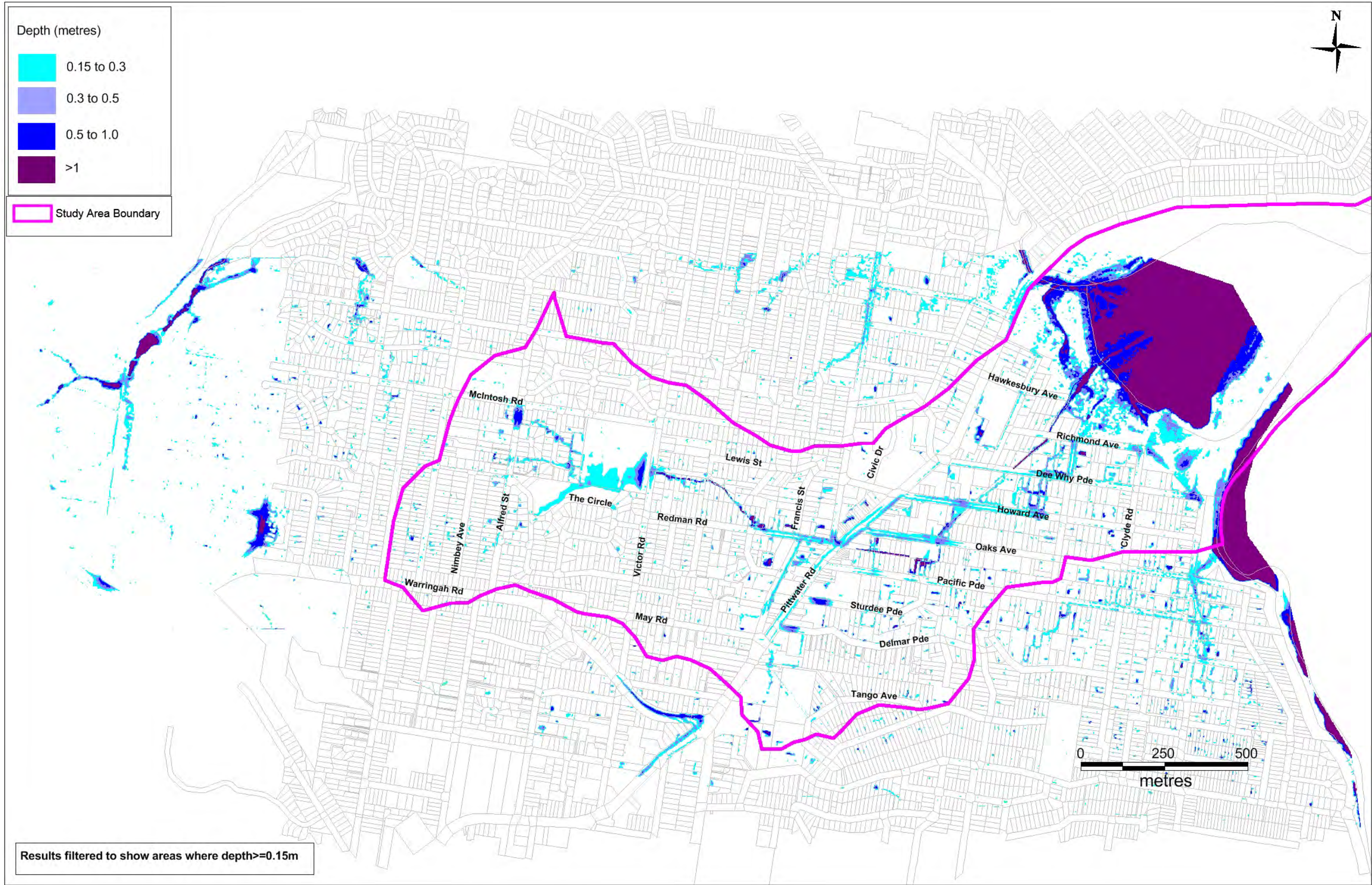
Figure 2-6 Peak Depths – Rainfall-On-Grid Model
