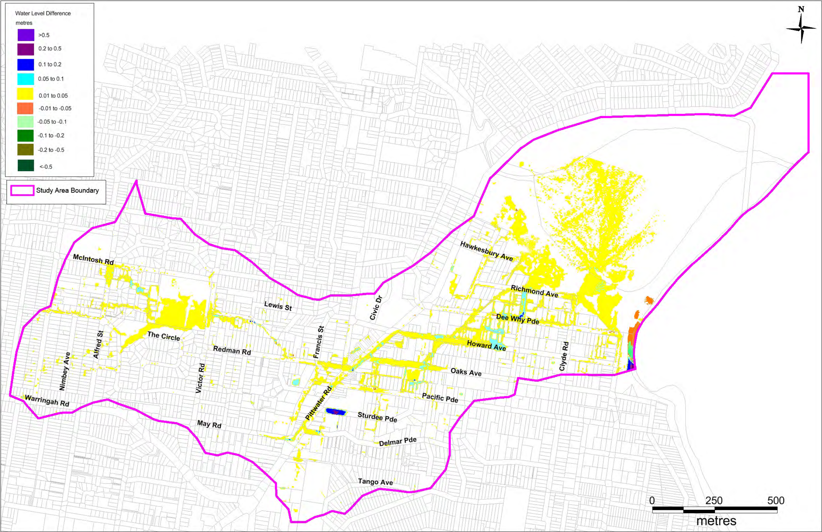
Figure 11-3 Rainfall Intensity Increase 10%
