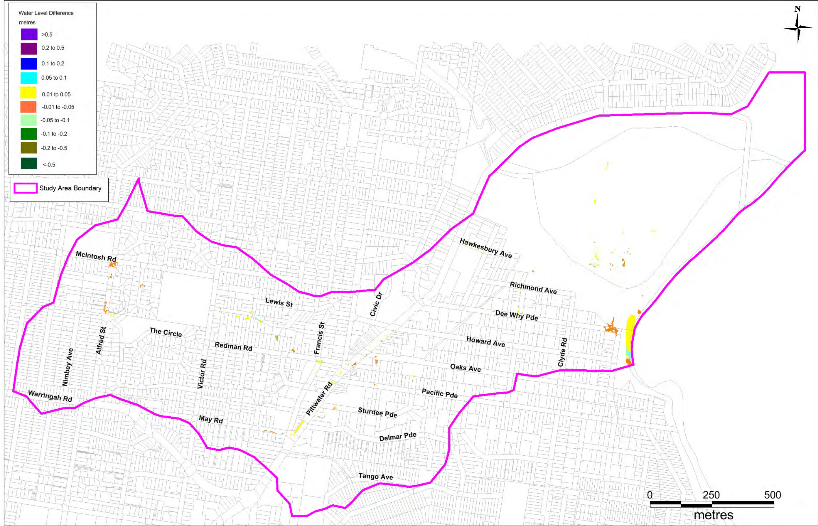
Figure 7-7 Sensitivity – Pervious Area Rainfall Losses +20%
