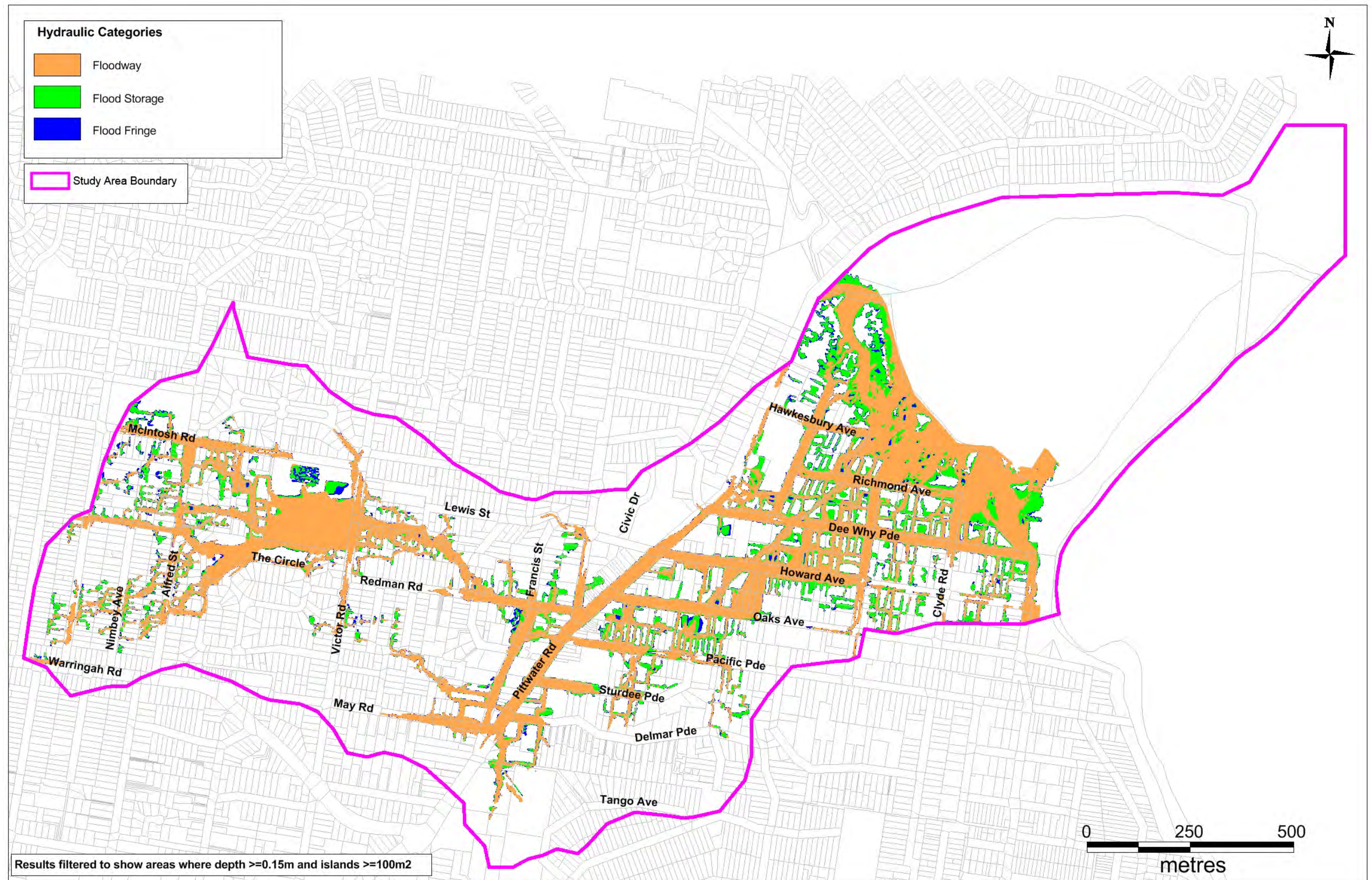
Figure 8-1 Hydraulic Categorisation PMF Event
