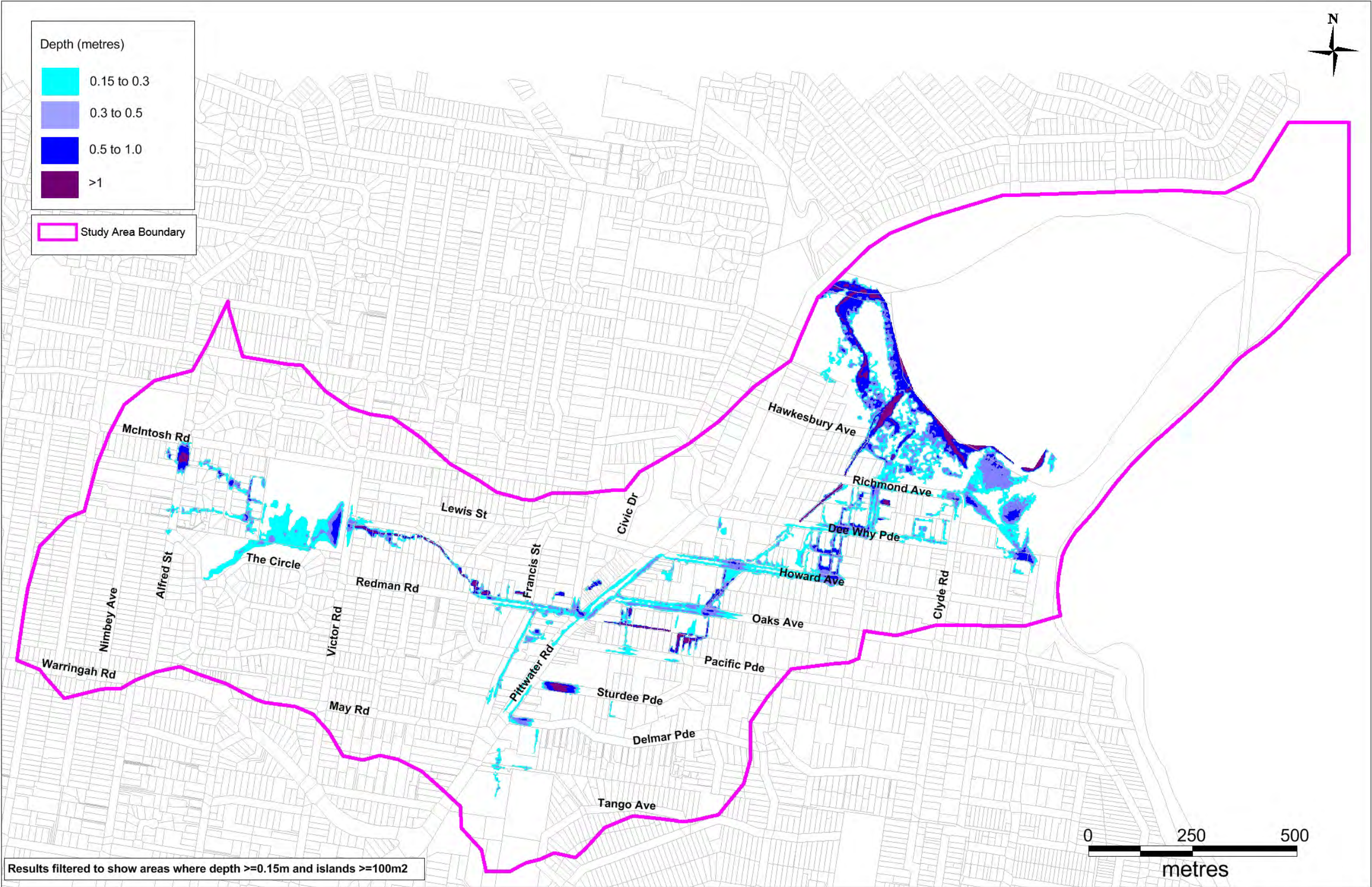
Figure 6-3 Design Event 0.1% AEP Peak Depth
