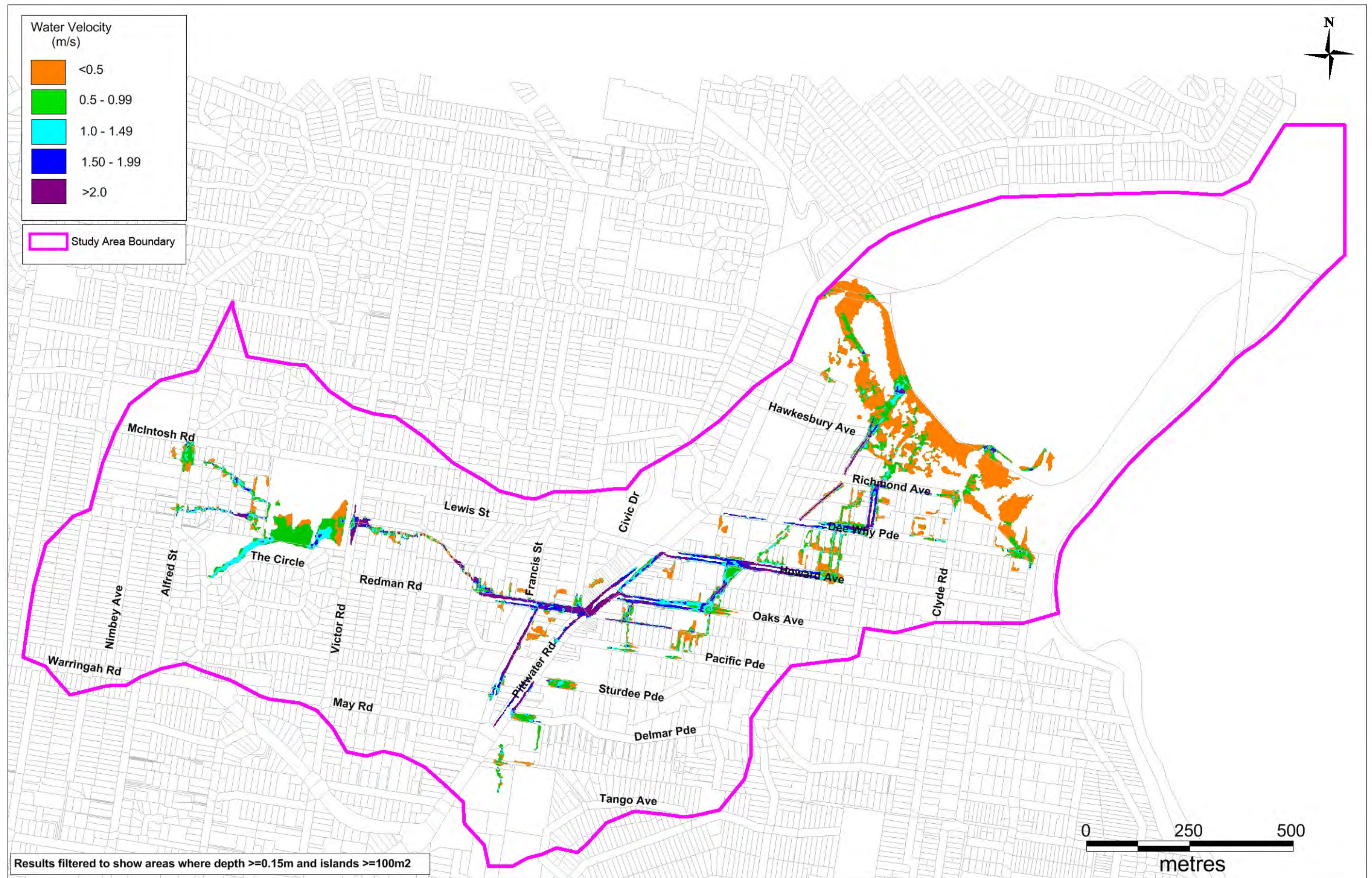
Figure 6-8 Design Event 1% AEP Peak Velocity
