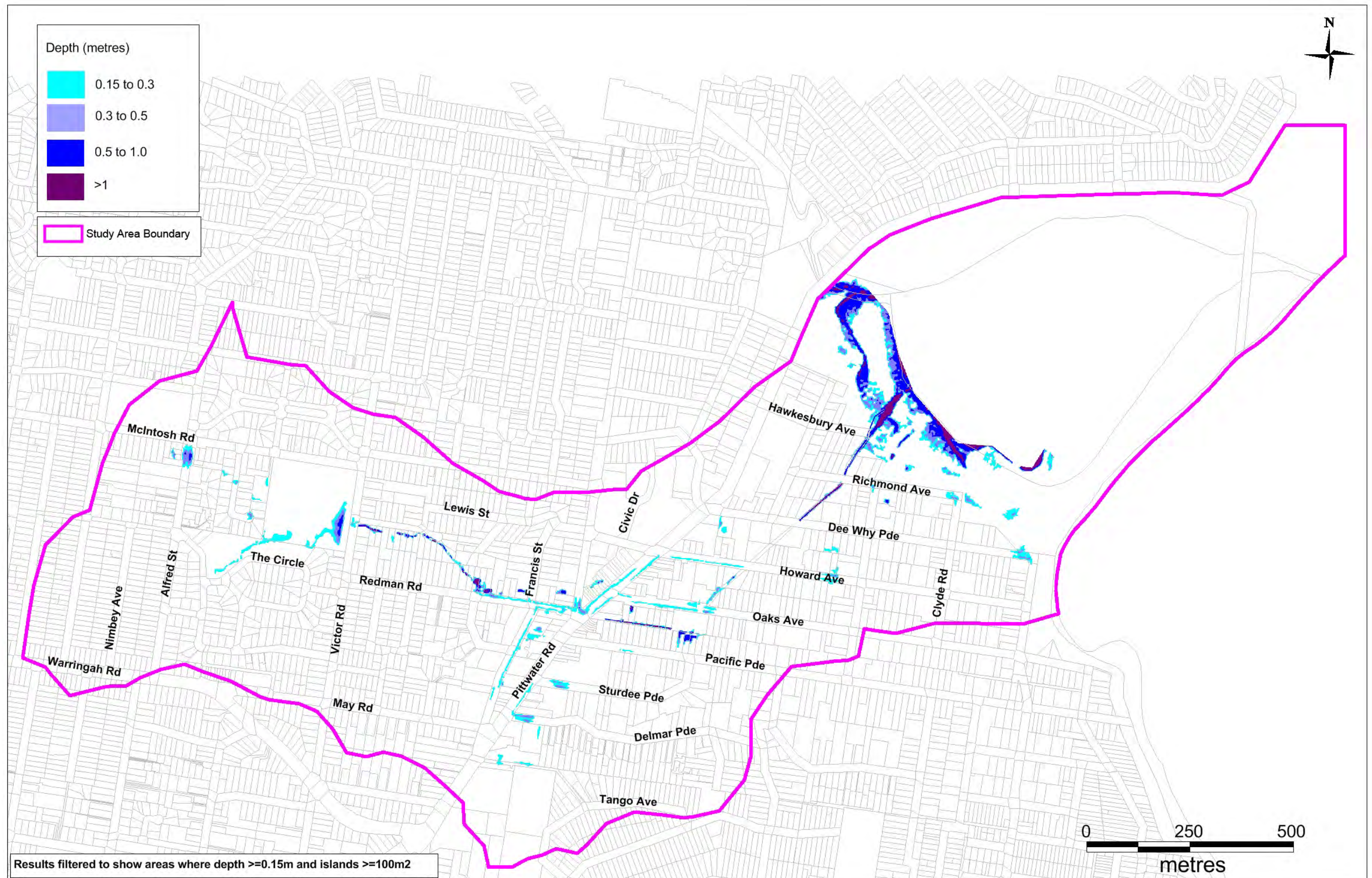
Figure 6-13 Design Event 5 Year ARI Peak Depth
