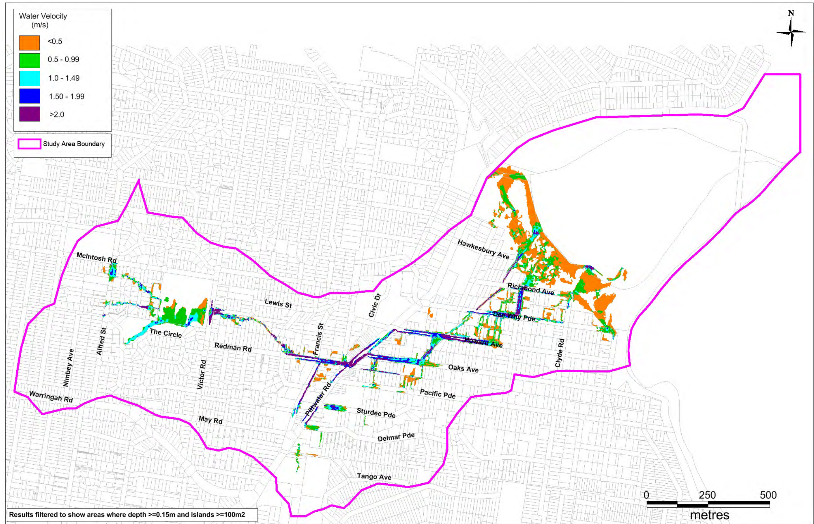
Figure 6-4 Design Event 0.1% AEP Peak Velocity
