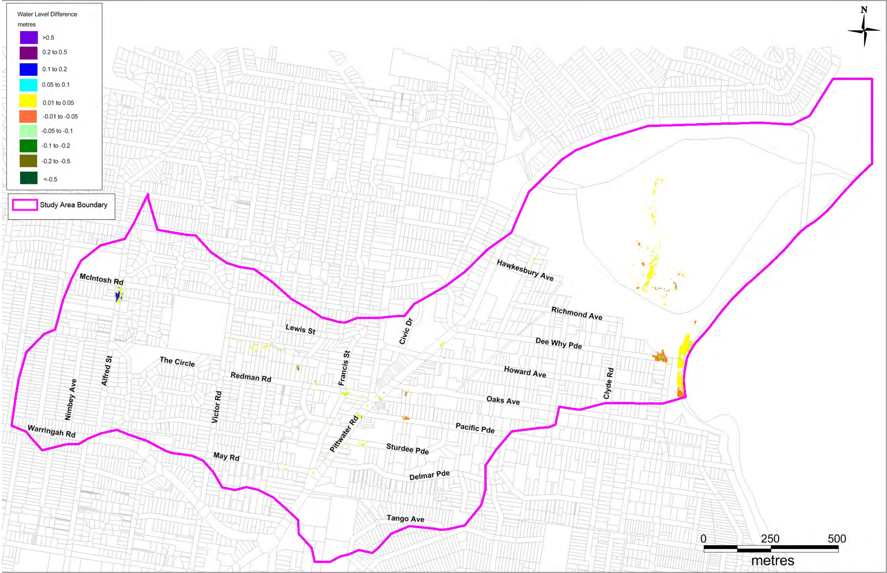
Figure 7-8 Sensitivity – Pervious Area Rainfall Losses -20%
