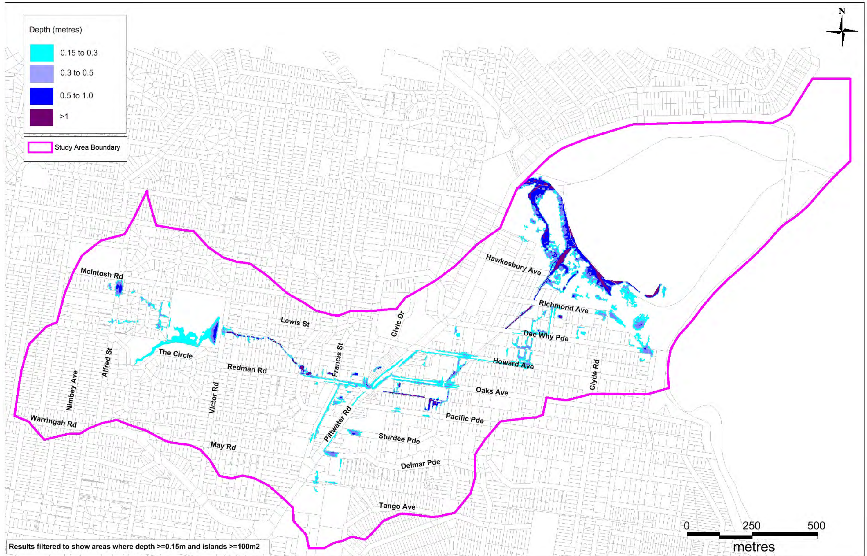
Figure 6-9 Design Event 5% AEP Peak Depth
