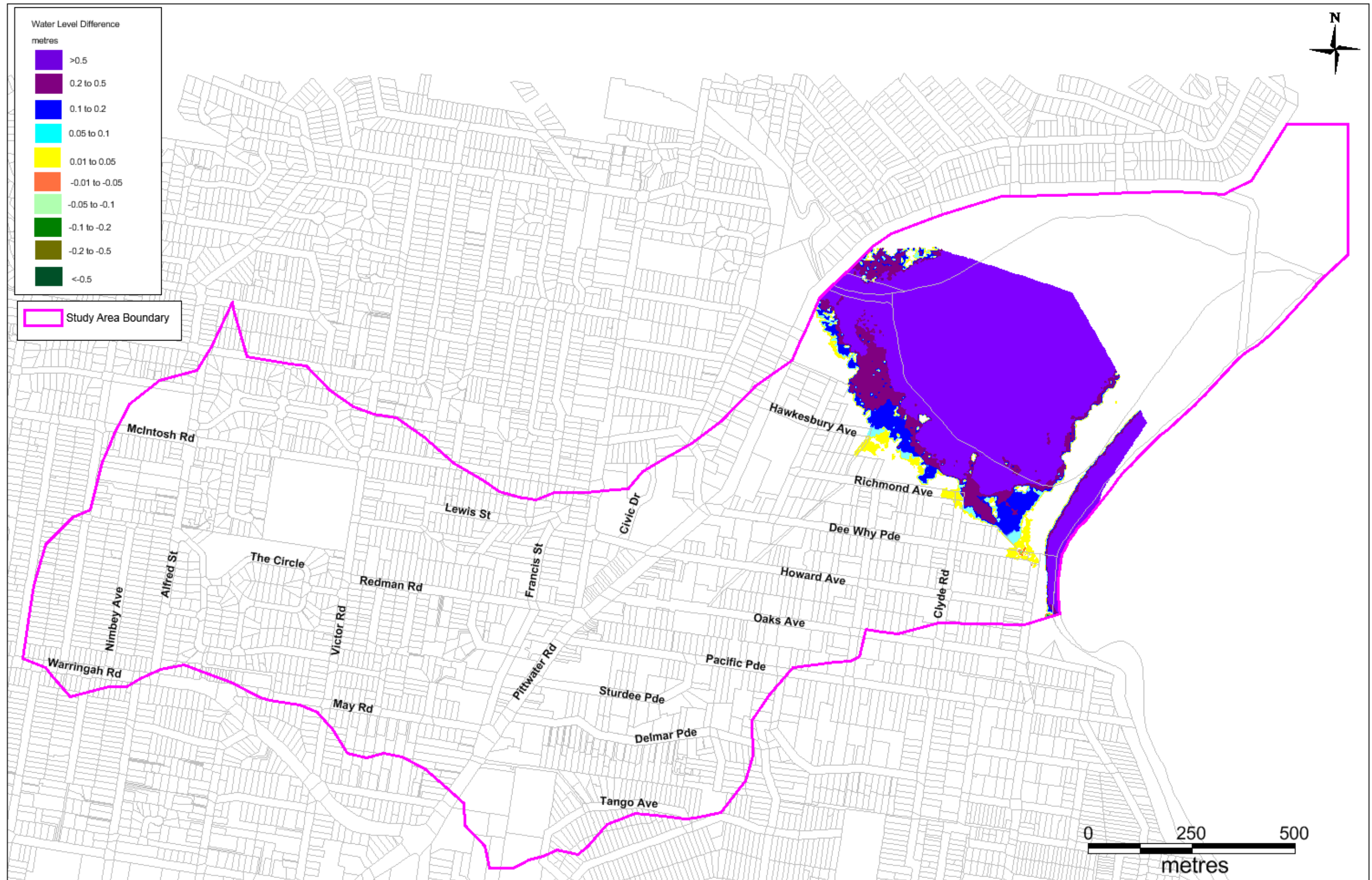
Figure 11-2 Sea Level Rise 0.9 m
