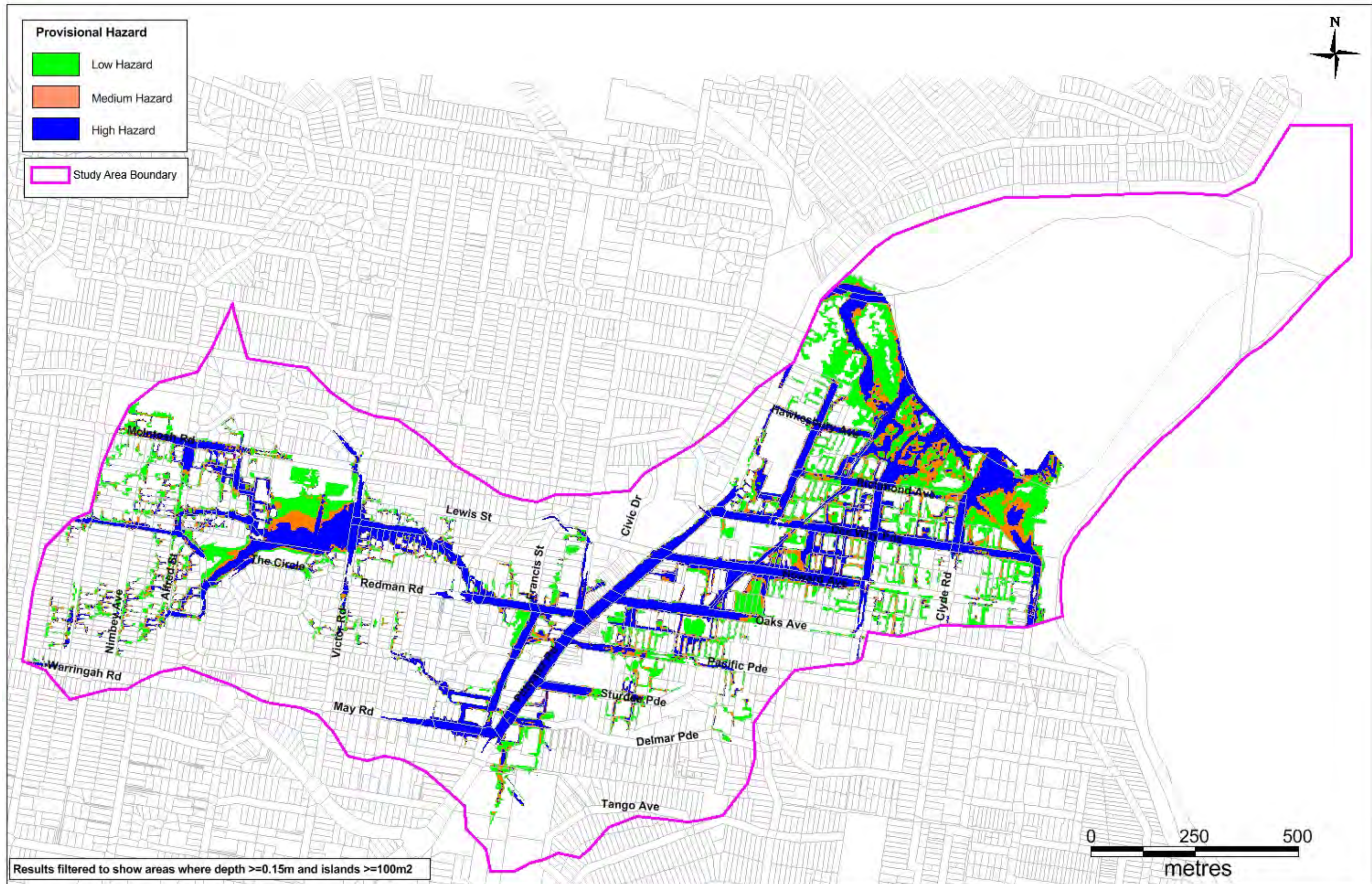
Figure 8-6 Provisional Hazard Classification PMF Event
