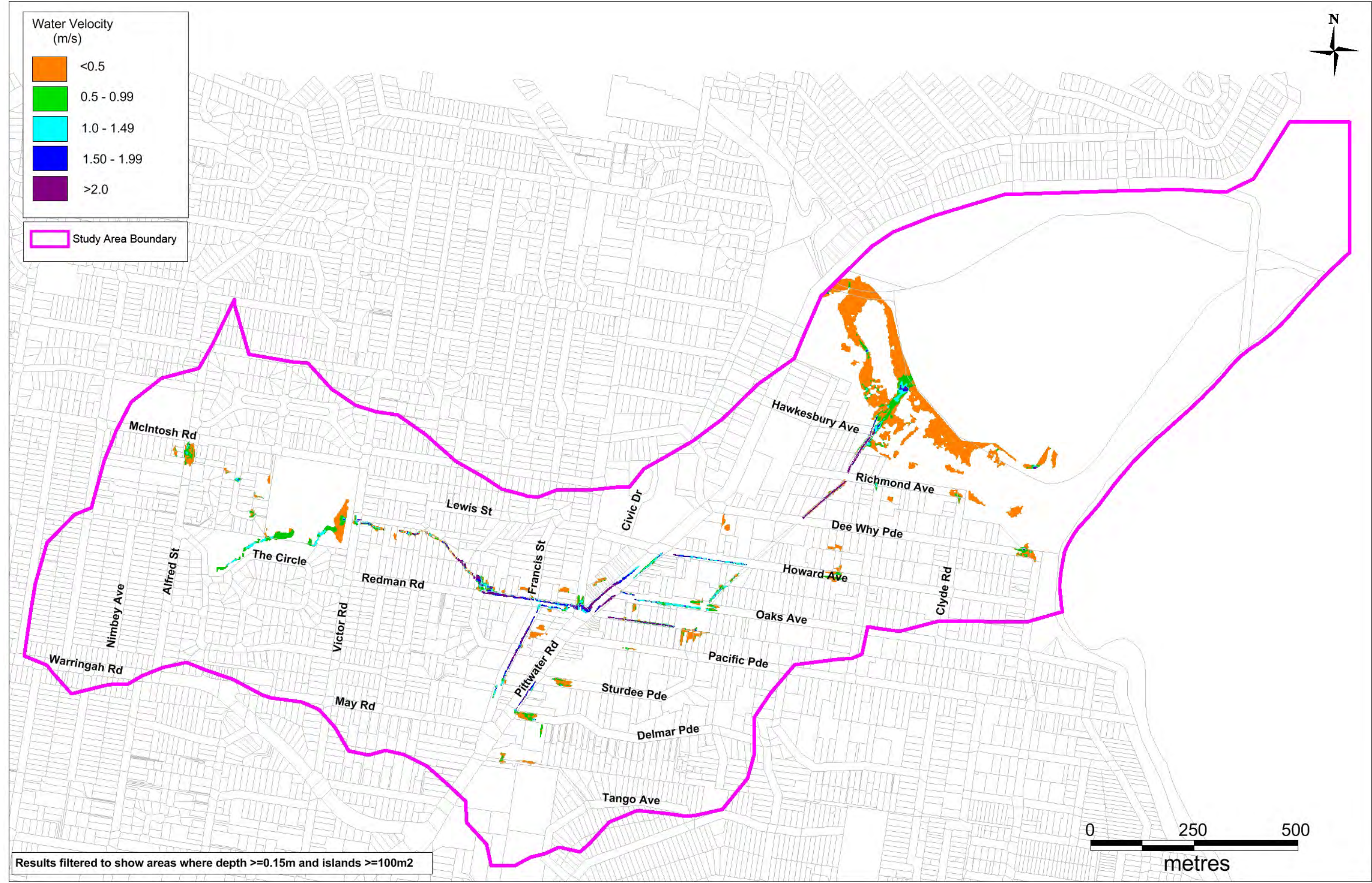
Figure 6-14 Design Event 5 Year ARI Peak Velocity
