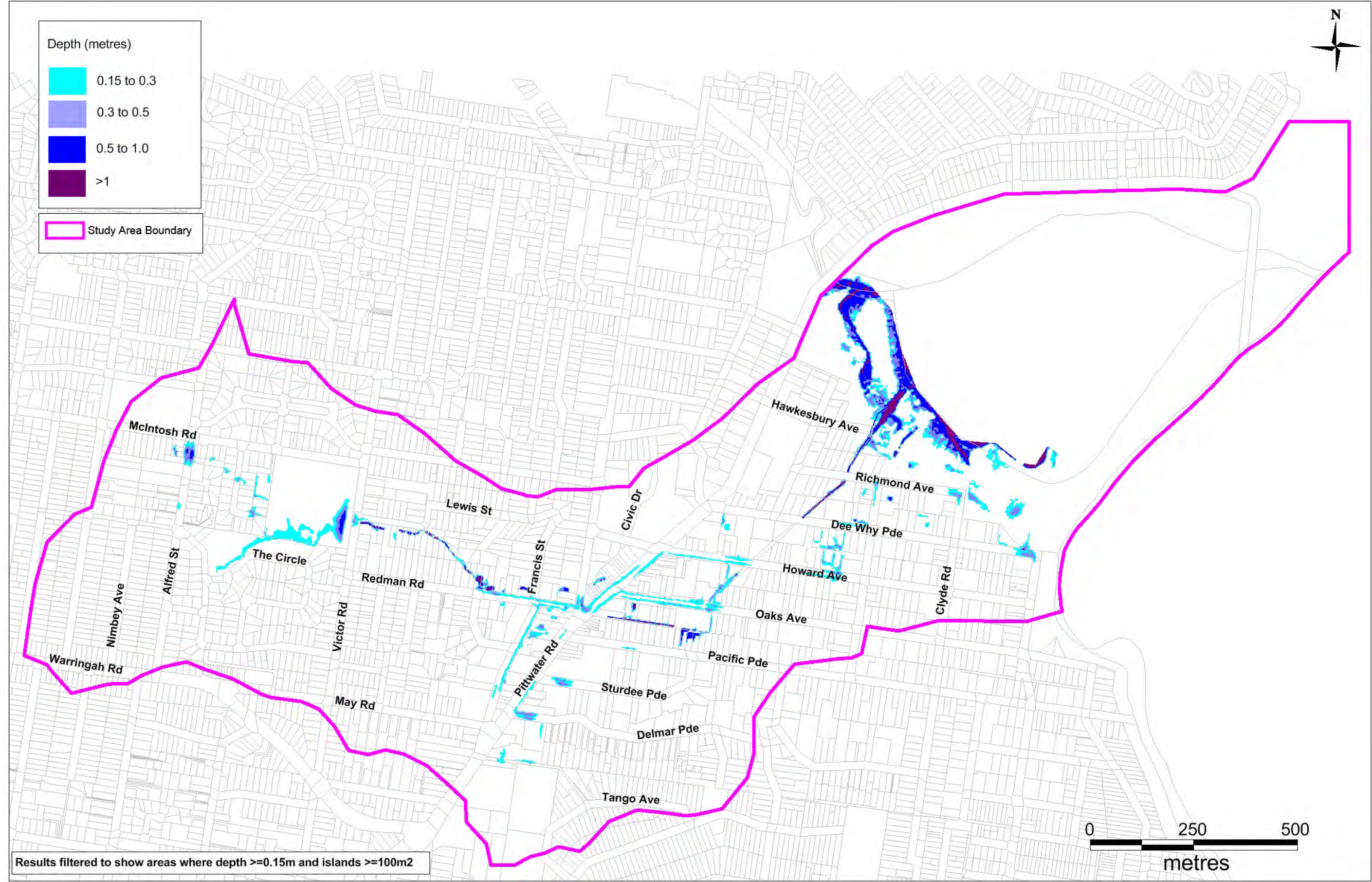
Figure 6-11 Design Event 10% AEP Peak Depth
